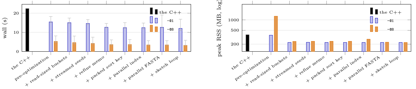
Figure 2: Every optimization, put back one at a time. The leftmost bar is the C++ itself; pre-optimization is this port with every ablatale change switched off (SHMAP_ABLATE), so the step between those two is the port and nothing else — the largest step in the figure, and the one the layered story does not cover. Each rung to the right switches exactly one more change back on, so adjacent rungs differ by one change and nothing else. The two series are the two thread counts, and the gap between them is row 4; row 8 is not ablatale, and the C++ is single-threaded so it has no -0N counterpart. Left: wall clock, median over 9 round-robin runs of the whole ladder, whiskers at min-max, so an unresolved step is visible as one. Right: peak resident set, log scale — one worker’s genome-sized accumulator hides under the index-build peak, -08 workers’ copies do not. Every rung’s mapping is byte-identical; the run fails otherwise. The C++ bar carries no -x (the C++ has no equivalent) while the rungs do, costing 1.06\times , so the first step is understated rather than flattered. Numbers and per-stage timers in figure_ablation.tsv ; the decomposition against the C++ in reconcile.tsv .
