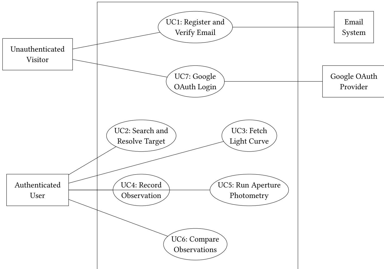
Figure 1: Use case diagram showing interactions for unauthenticated and authenticated users.
