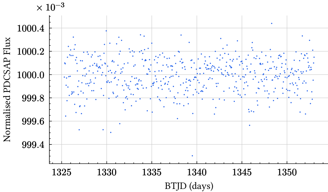
Figure 9: TESS Sector 1 light curve for pi Mensae. Transit dips of \sim 300 ppm are visible at \sim 6.27 -day intervals.
