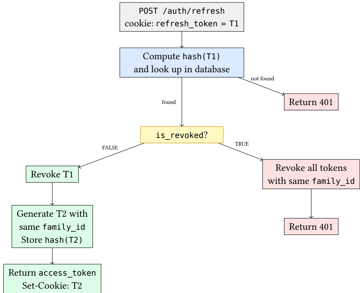
Figure 6: Refresh token rotation with family-based reuse detection.
