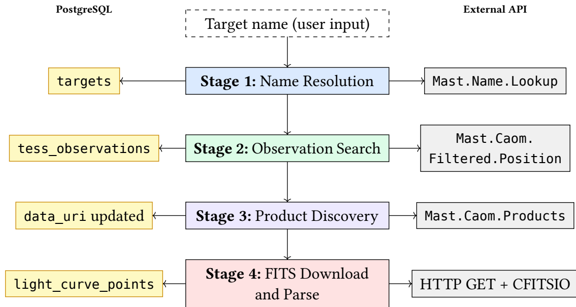
Figure 4: Four-stage TESS data ingestion pipeline. Each stage calls a MAST API service (right) and persists its output to PostgreSQL (left).
