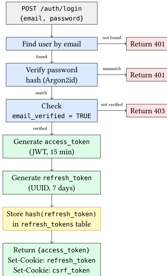
Figure 7: Login sequence showing token generation and cookie setting.
