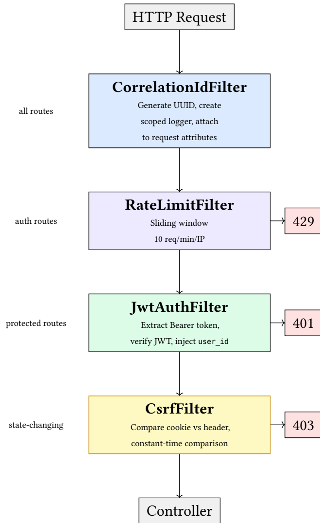
Figure 8: HTTP middleware filter chain. Each filter can short-circuit the request with an error response.
