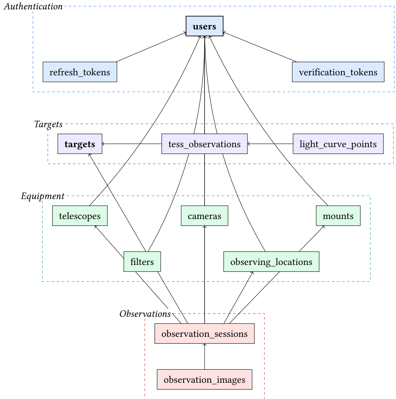
Figure 3: Entity-relationship diagram of the Nyx database schema. Arrows indicate foreign key references (child \rightarrow parent). Tables are colour-coded by domain: authentication (blue), targets (purple), equipment (green), and observations (red). All equipment tables reference users via user_id . The observation_sessions table references users, targets, and equipment tables.
