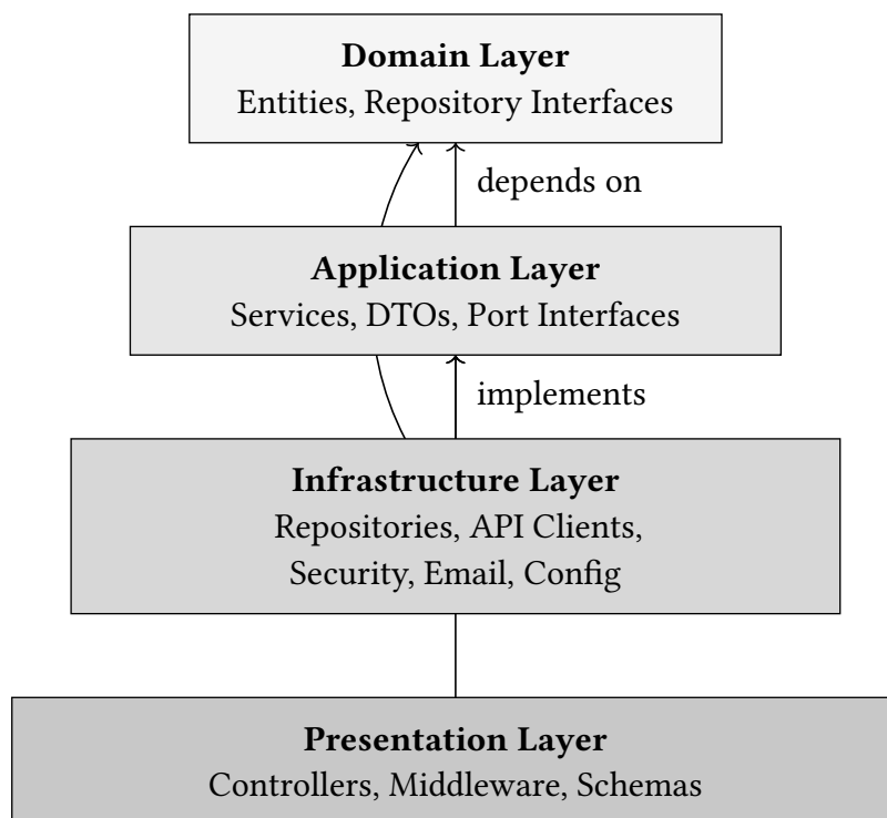
Figure 2: Clean architecture layers of the Nyx backend. Dependencies point strictly inward.
