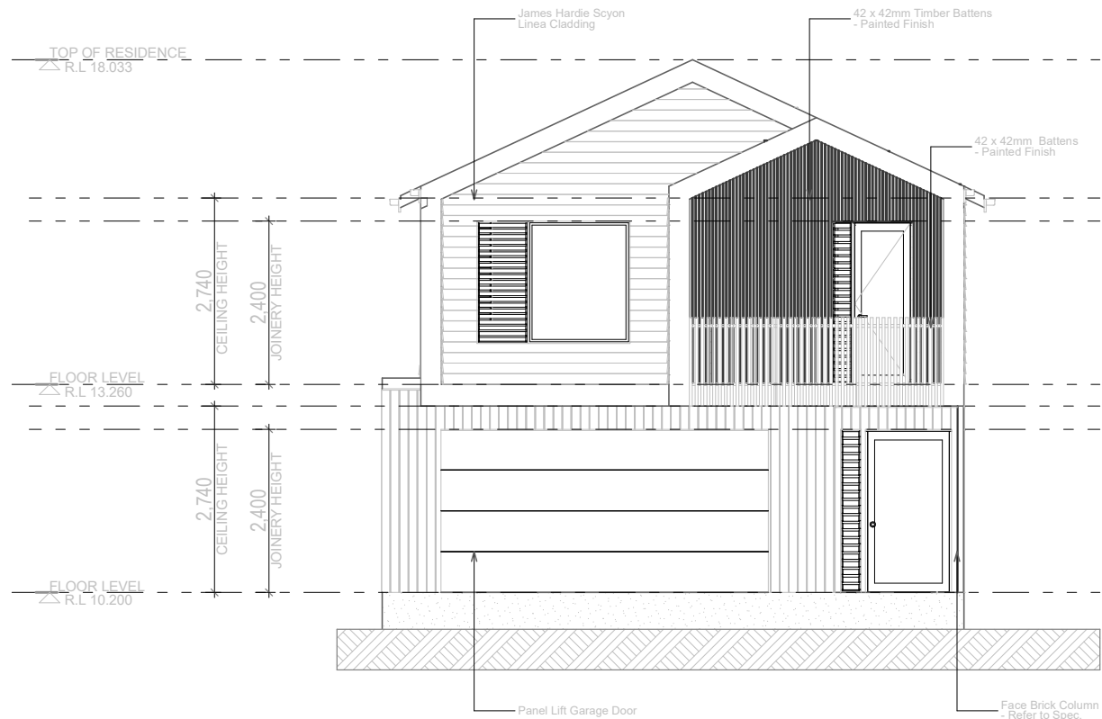
EAST ELEVATION
