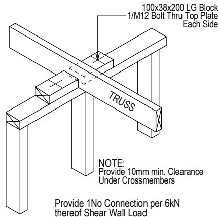
TRUSS CONNECTION TO INTERNAL SHEAR WALL TRUSSES NORMAL TO WALL
