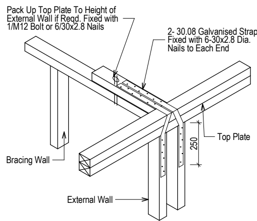
PERPENDICULAR TO WALL PROVIDE TWO CONNECTIONS FOR EVERY 1.2m LENGTH OF BRACING WALL
