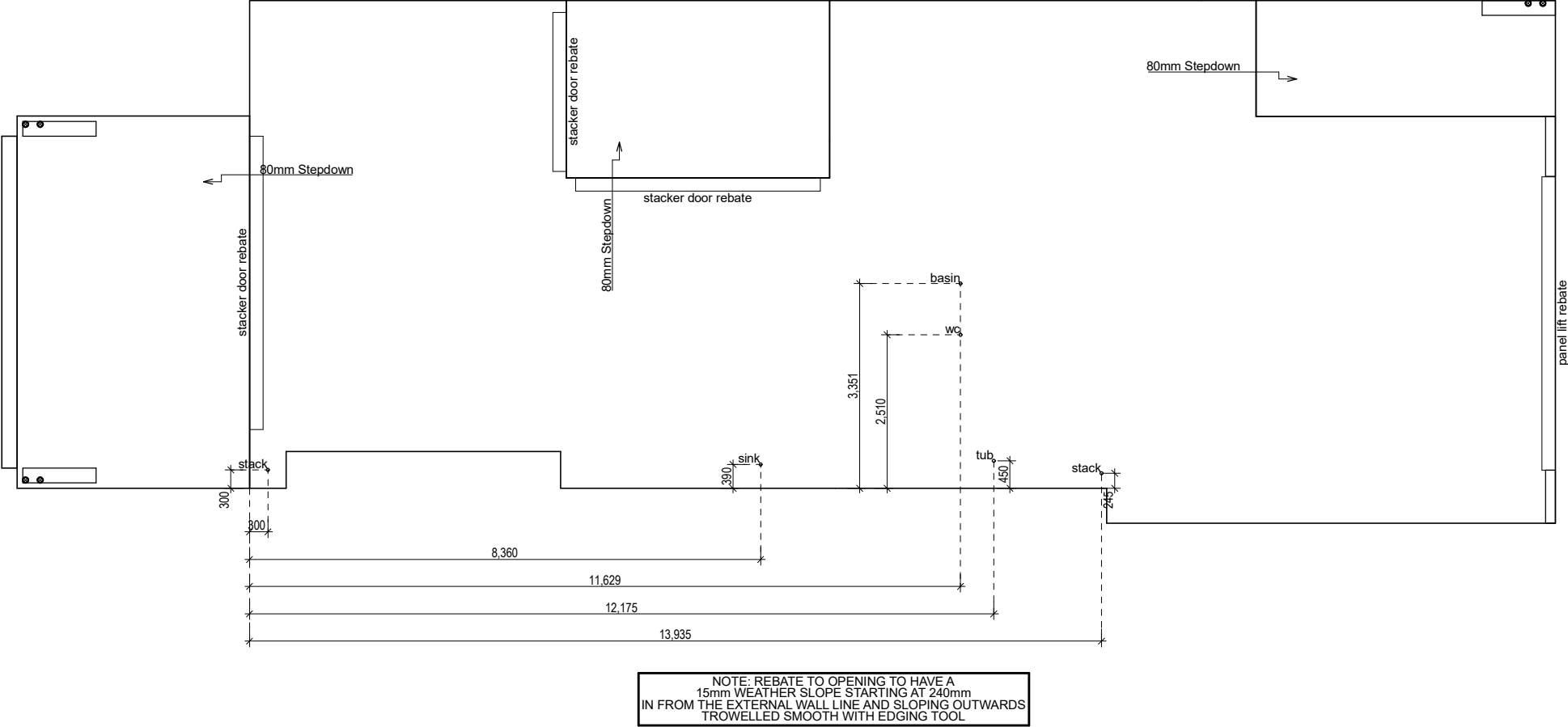
SLAB PENETRATION PLAN
