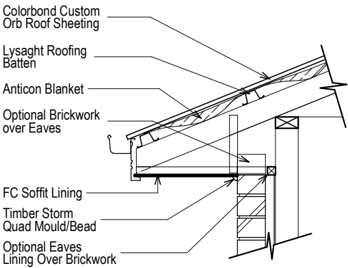
BOXED EAVES DETAIL - BRICK VENEER
