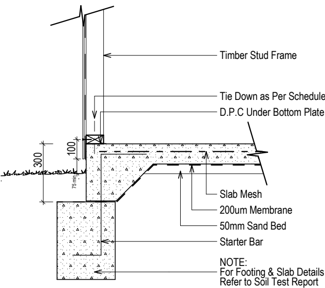
TIMBER FRAME W/ FC CLADDING OR WEATHERBOARDS - SLAB ON GROUND
