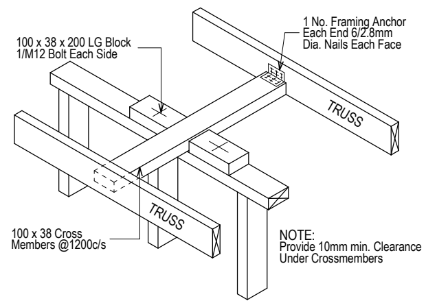
TRUSS CONNECTION TO INTERNAL SHEAR WALL TRUSSES PARALLEL TO WALL
