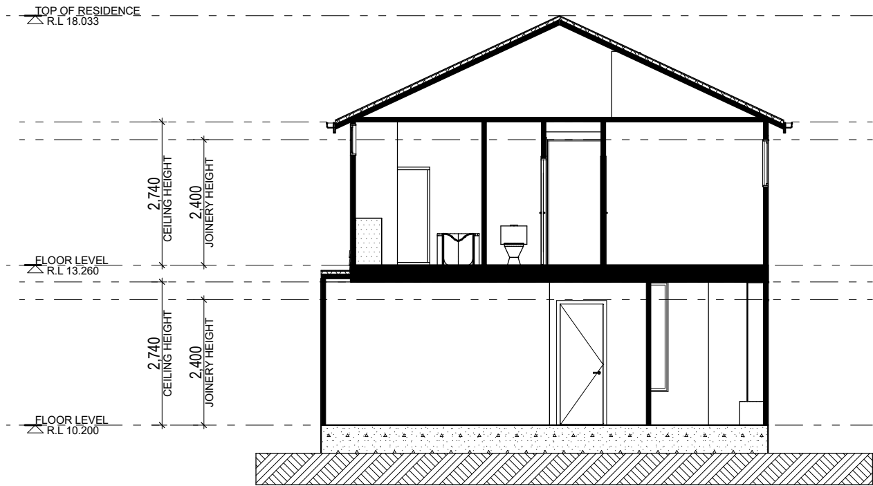
SECTION I-I
