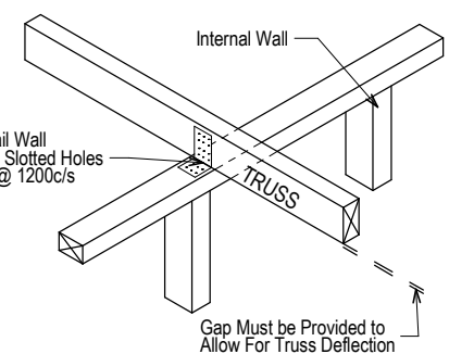
NON LOADBEARING WALL PERPENDICULAR TO TRUSSES
