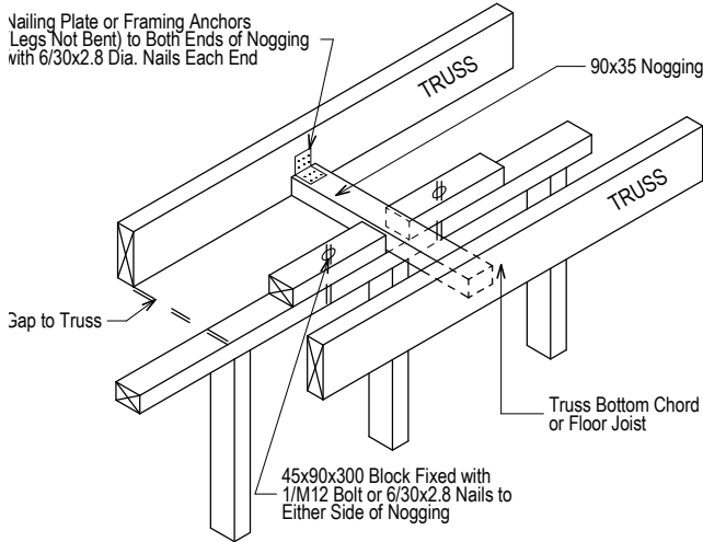
PARALLEL TO TRUSS PROVIDE TWO CONNECTIONS FOR EVERY 1.2m LENGTH OF BRACING WALL
