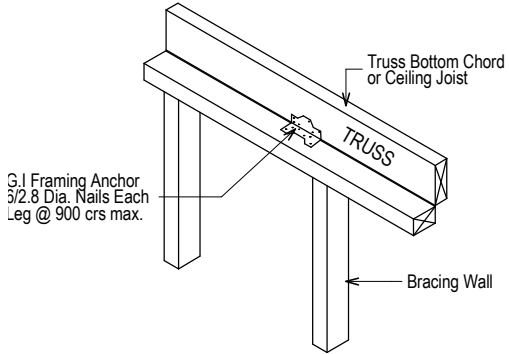
PARALLEL TP TRUSSES OR CEILING JOISTS PROVIDE TWO CONNECTIONS FOR EVERY 1.2m LENGTH OF BRACING WALL
