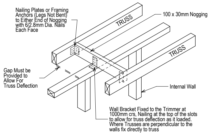
NON LOAD BEARING WALL PARALLEL TO TRUSSES
