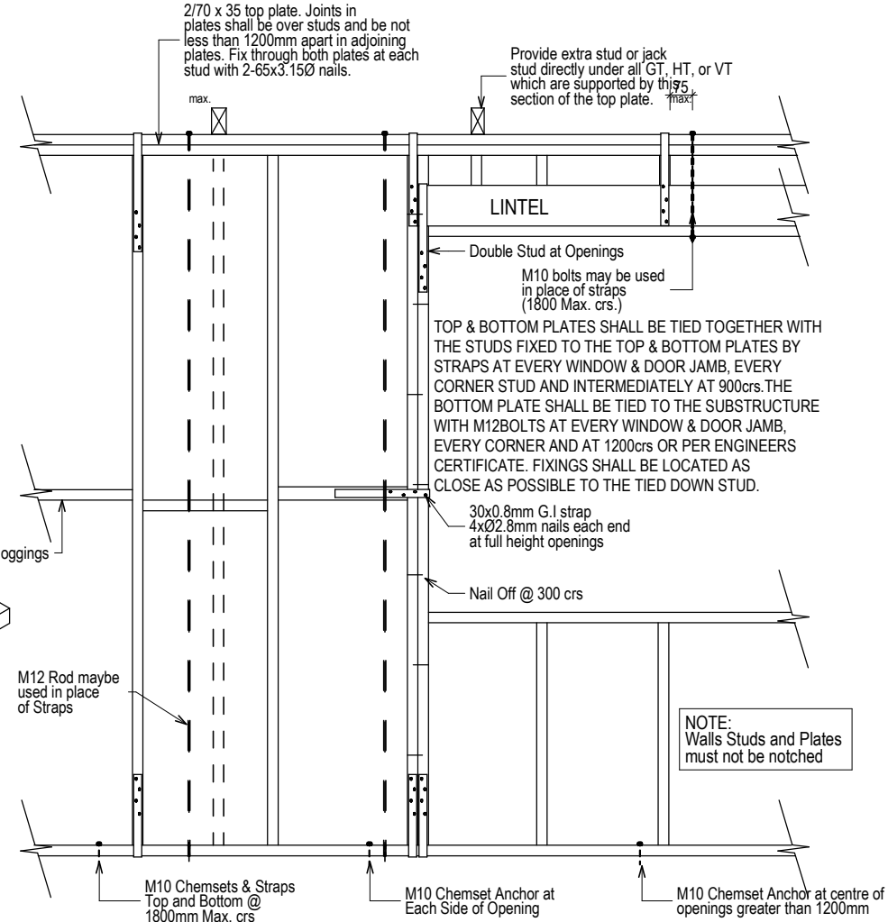
TYPICAL TIEDOWN DETAIL
