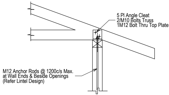
TRUSS HOLD DOWN DETAIL
