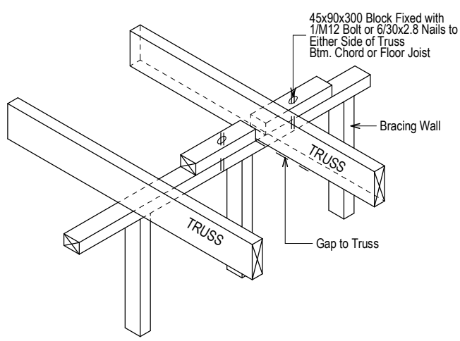
PERPENDICULAR TO TRUSS
