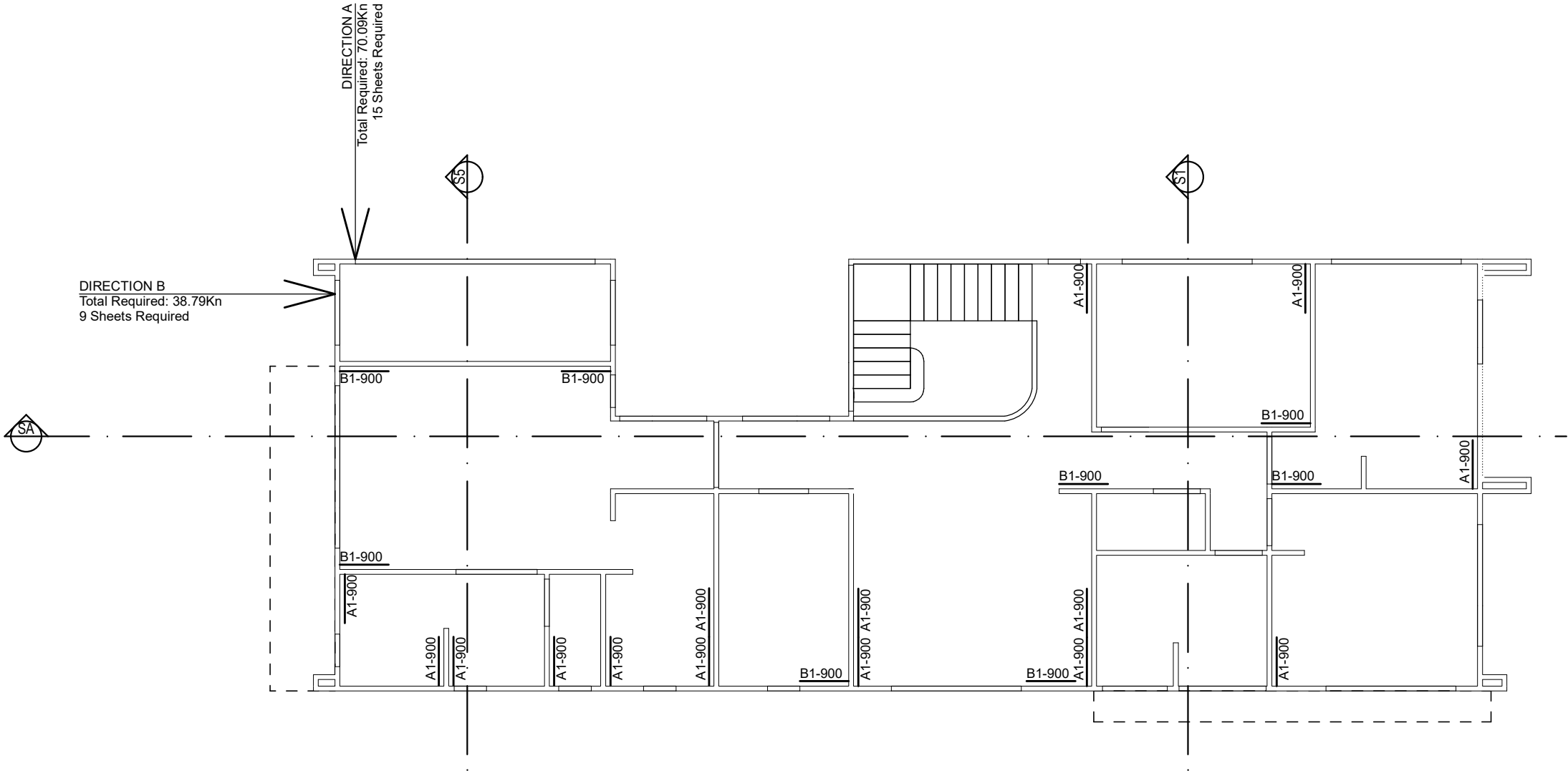
BRACING UPPER
