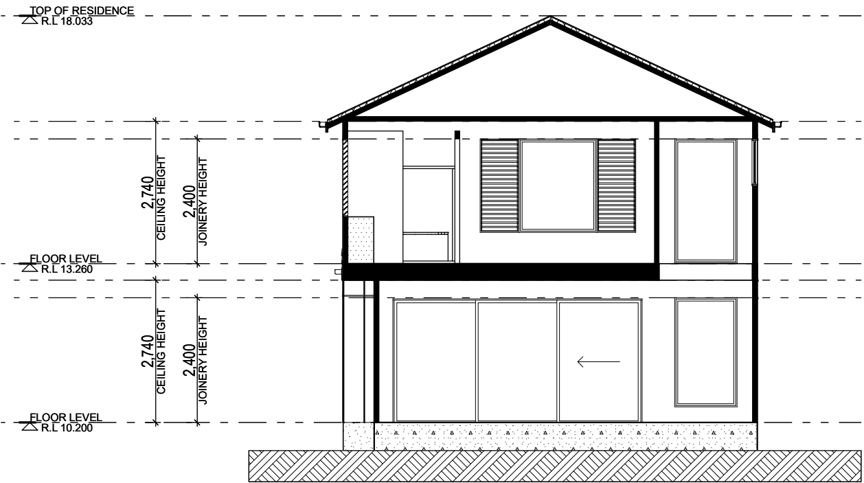
SECTION 2-2 1:100
