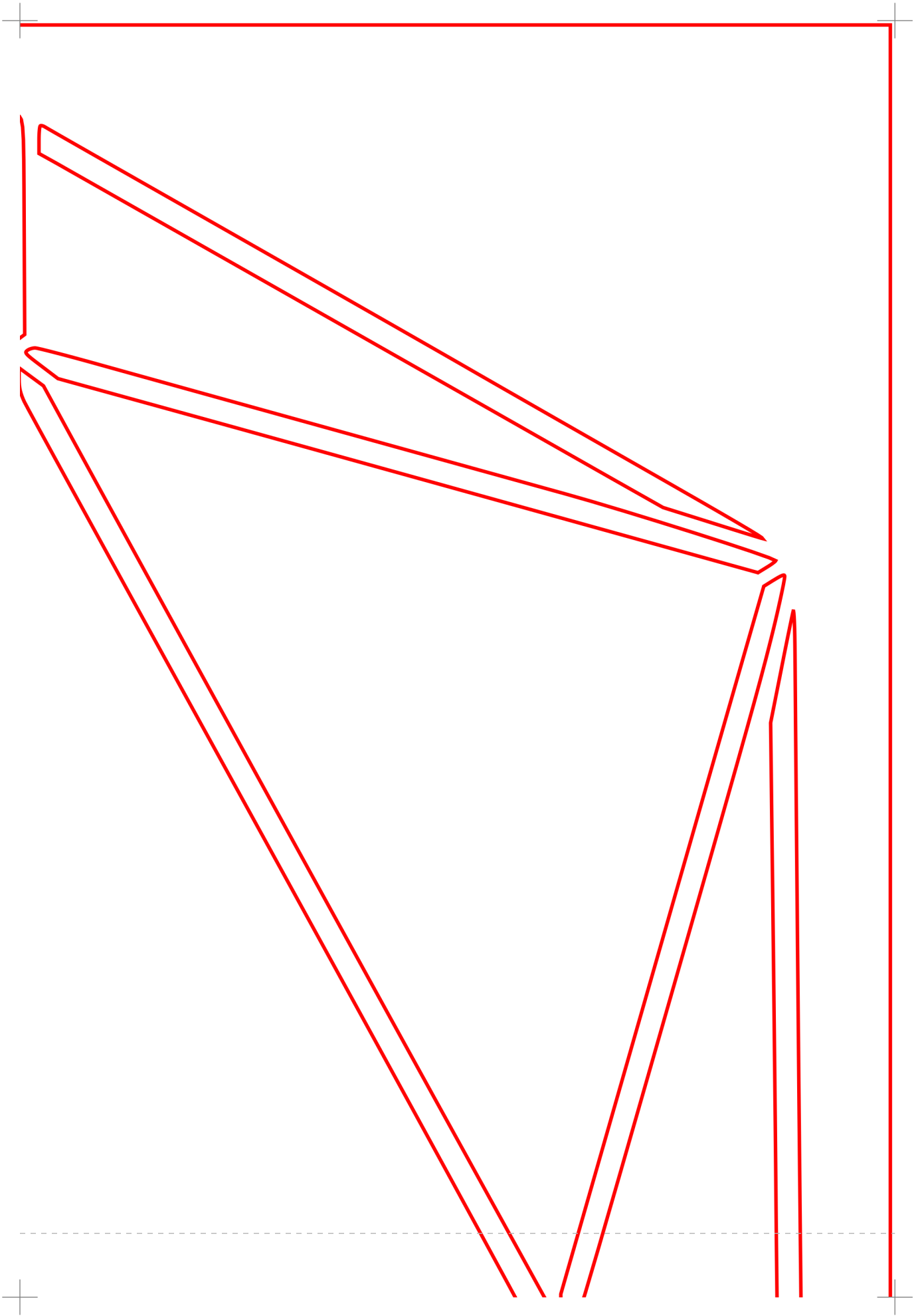
Tile (2,1) of (2,2)
