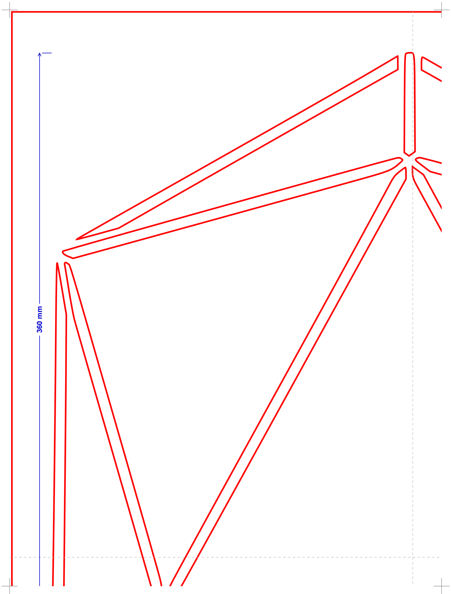
Tile (1,1) of (2,2)
