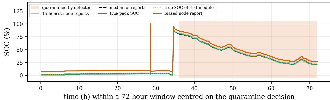
(b) N5: node broadcasting a +5 % firmware bias
