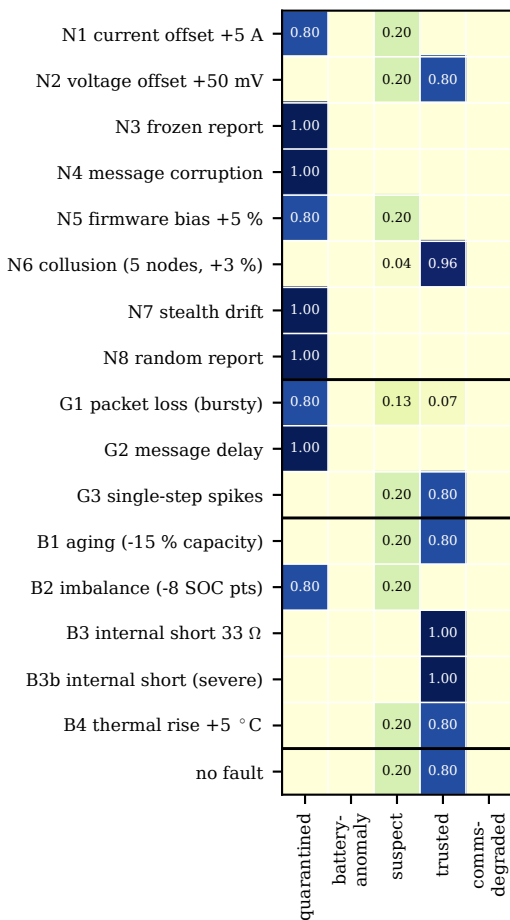
(a) round-1 detector (no router, no freshness)
