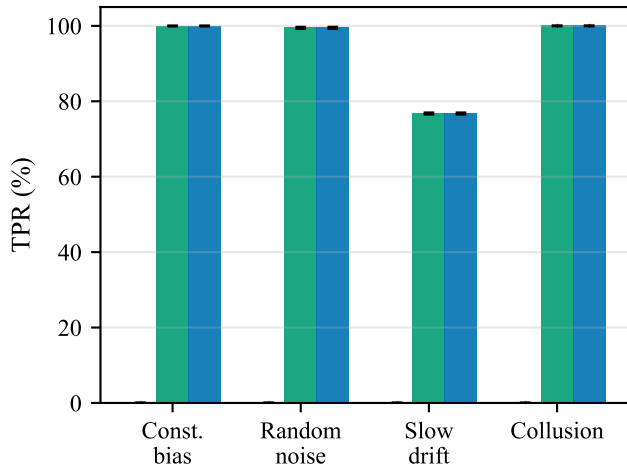
(b) True positive rate
