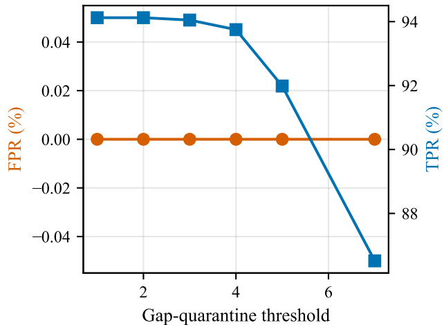
(b) ABR-PINN gap detector
