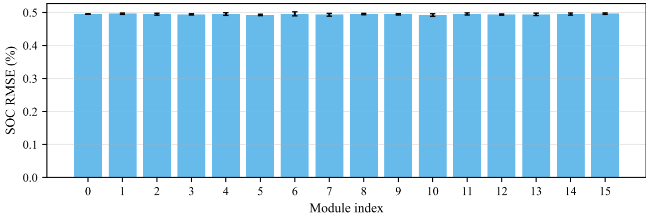
Per-module SOC accuracy under min/max interpolation
