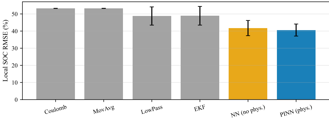
Local SOC estimator: PINN vs simple filters ( \text{LiFePO}_4 )
