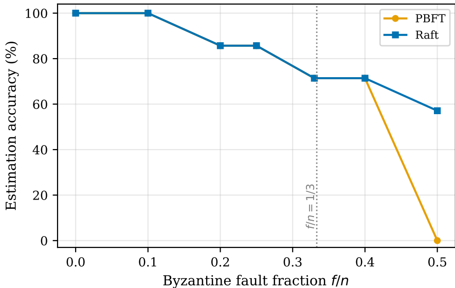
Decided-value accuracy vs ground truth ( n = 7 , equivocation)
