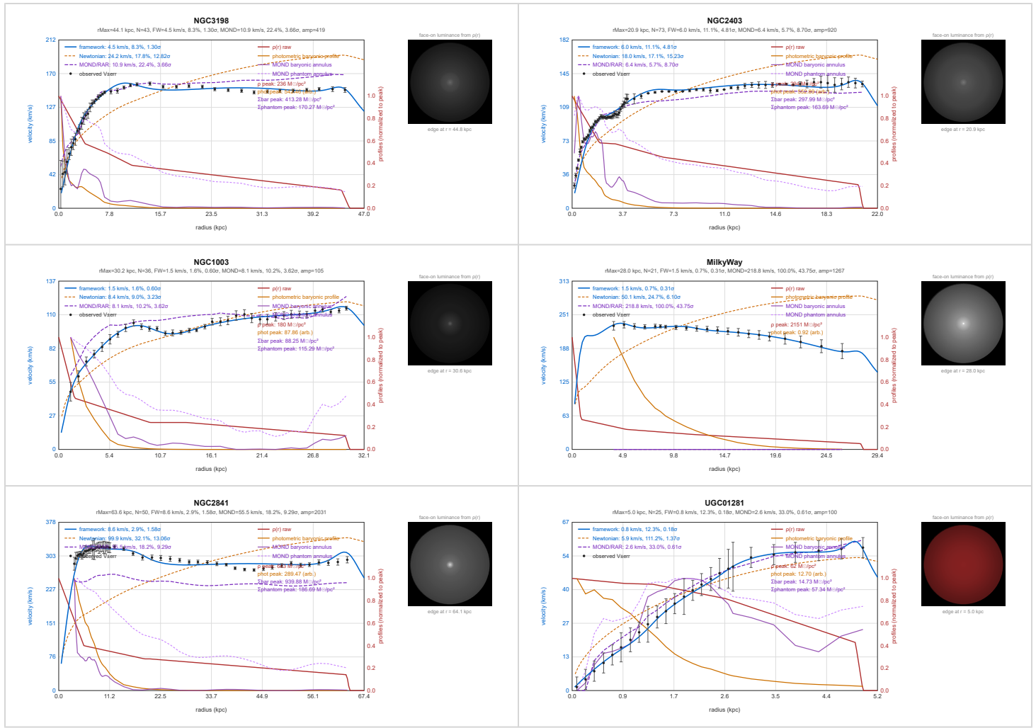
Figure 2. Representative framework rotation-curve fits and stress cases. Each panel shows the observed rotation data, the displacement-framework fit, comparison curves, and the fitted bounded occupation profile. The examples are selected to show ordinary disk recovery, lower-mass behavior, a local anchor, and the inner-rise stress class rather than to show only the lowest-RMS cases.
