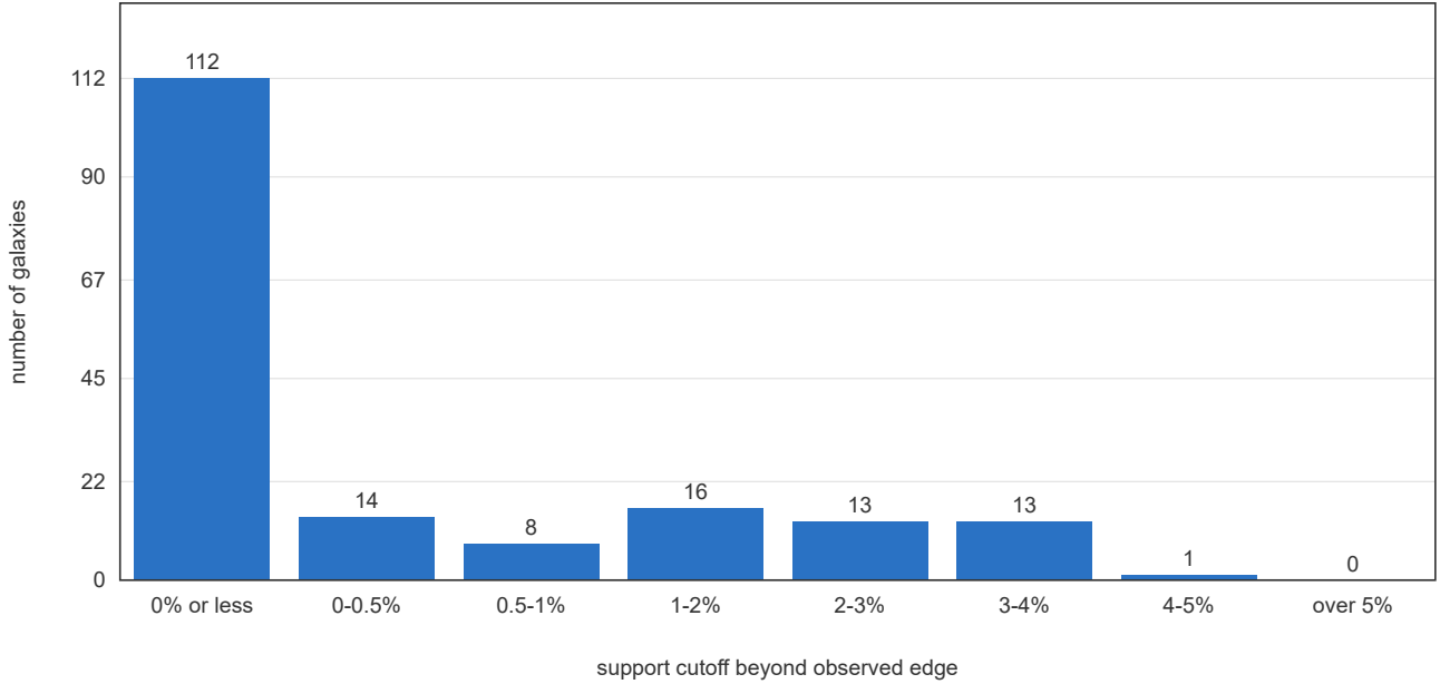
Figure 3. Outer cutoff distribution of fitted support profiles. The figure shows the fitted support cutoff beyond the outermost measured rotation point, zoomed over the 0–5% extension regime. File: AI/Revised/fig/galaxy-fits/fits/_aggregate_edge_bounded.svg .
