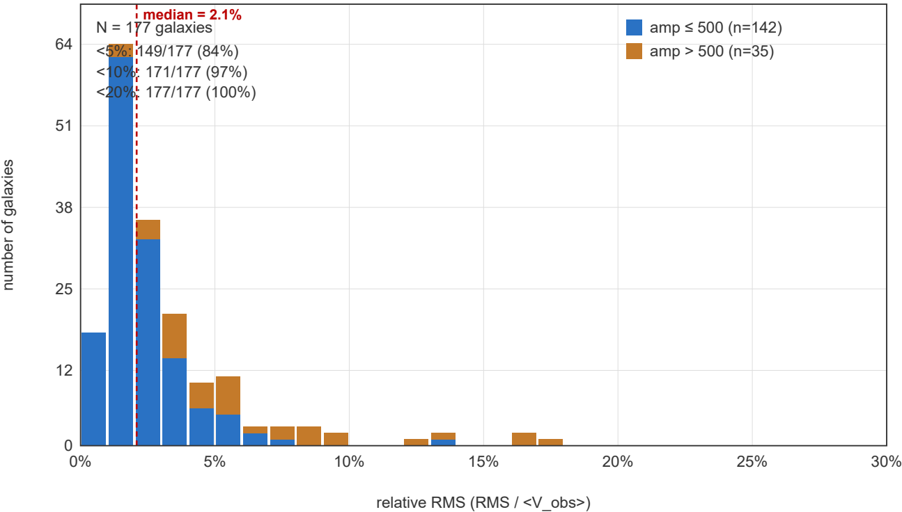
Figure 1. Distribution of relative RMS ( \text{RMS} / \langle V_{\text{obs}} \rangle ) across the 177-galaxy sample. The median is 2.09%; the high-amp cohort ( \text{amp} > 500 , where the evolutionary fit is more likely to settle in local optima) is stacked separately. File: fig/galaxy-fits/fits/_aggregate_rms_distribution.svg .
