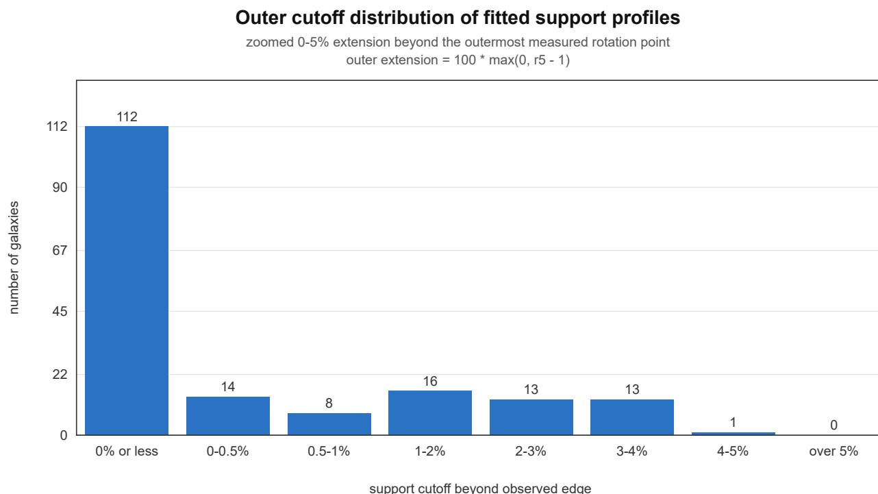
Figure 3. Outer cutoff distribution of fitted support profiles. The figure shows the fitted support cutoff beyond the outermost measured rotation point, zoomed over the 0–5% extension
