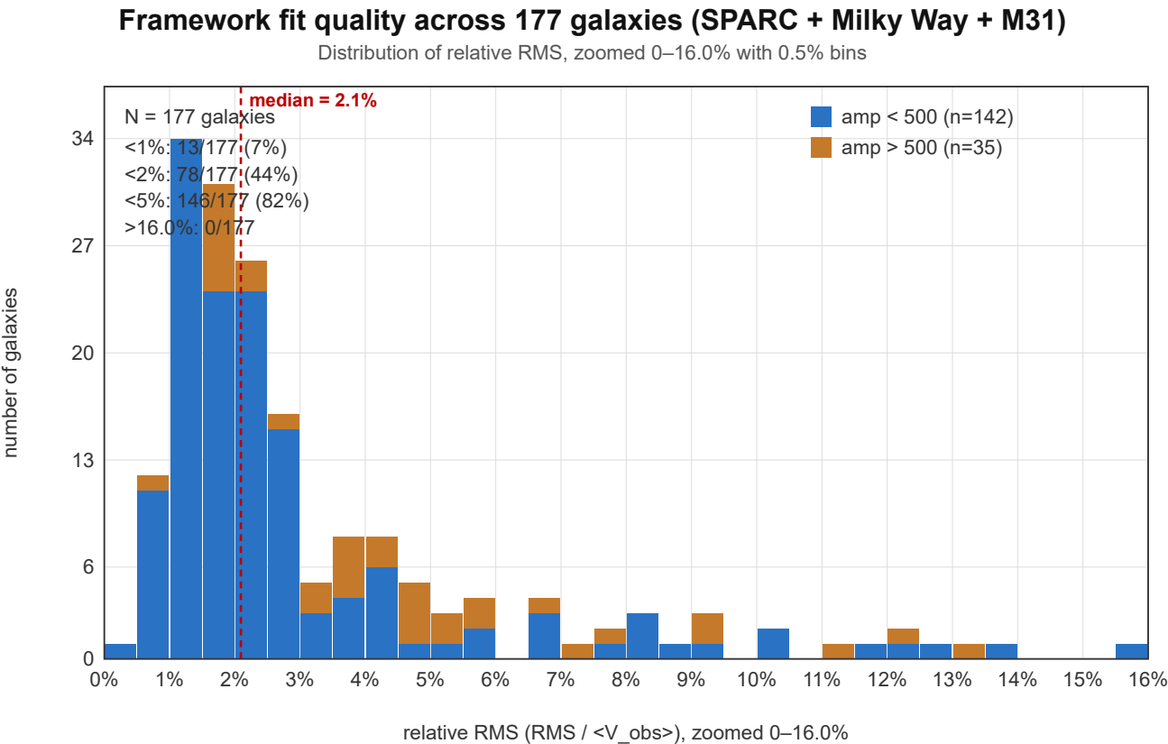
Figure 1. Distribution of relative RMS ( \text{RMS} / \langle V_{\text{obs}} \rangle ) across the 177-galaxy sample. The median is 2.09%. The stacked coloring follows the renderer's internal amp grouping, but amp is a slider-range normalization rather than a separate physical parameter. File: AI/Revised/fig/galaxy-fits/fits/_aggregate_rms_distribution.svg .
