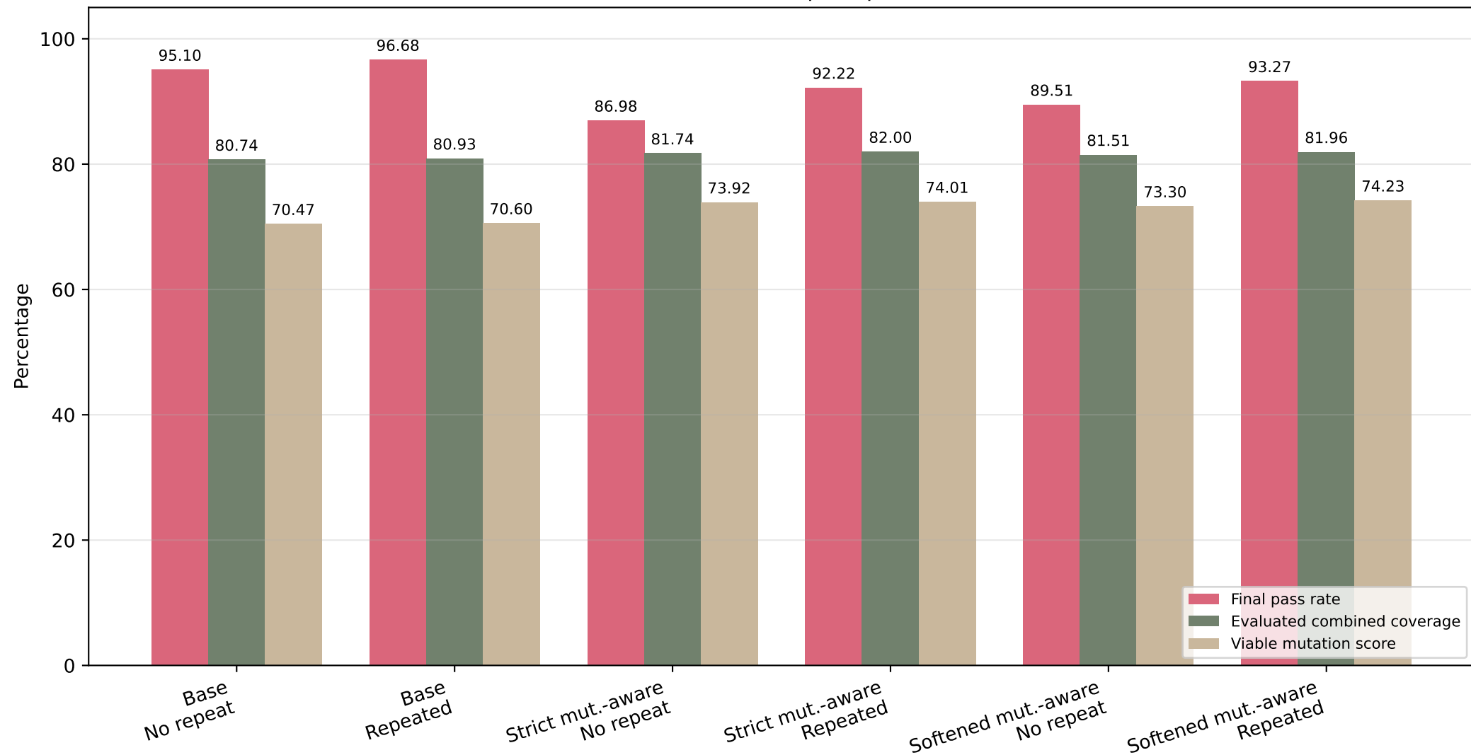
Qwen/Qwen3.5-27B prompt variants
