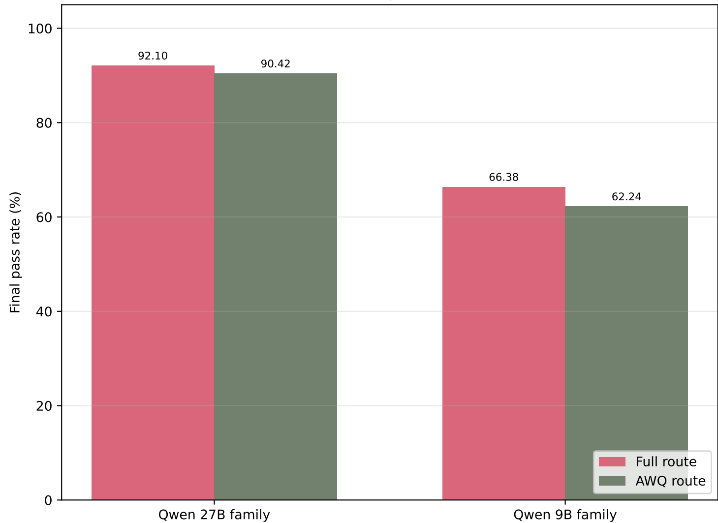
Matched full vs AWQ-quantised Qwen routes
