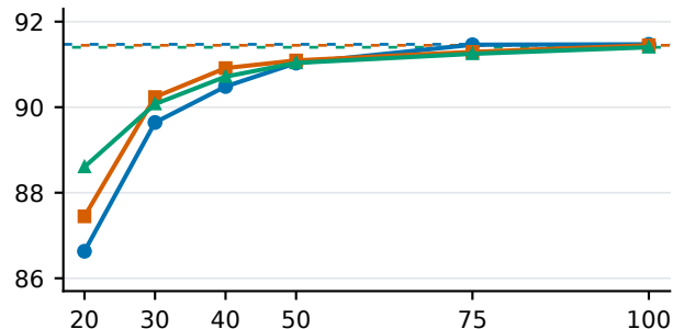
RULER 8K
