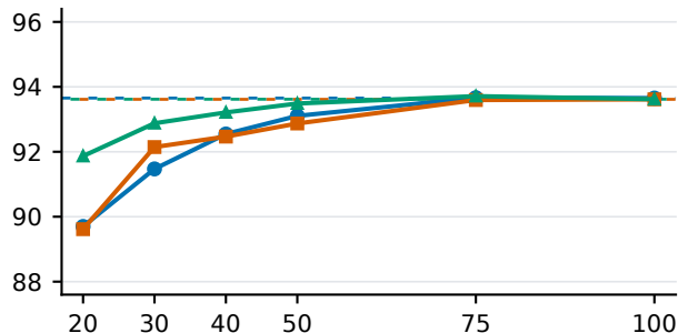
RULER 64K
