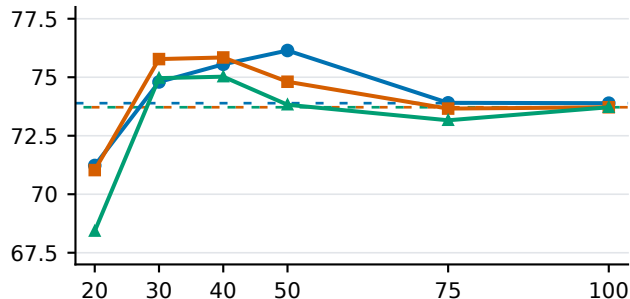
RULER 64K
