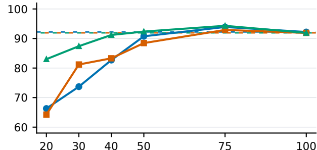
Multi-values NIAH
