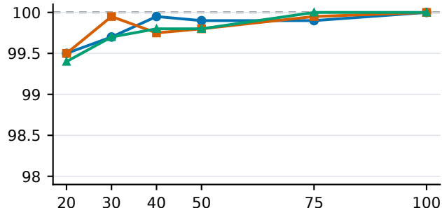
Multi-queries NIAH
