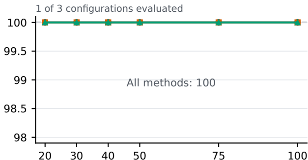
Single NIAH
