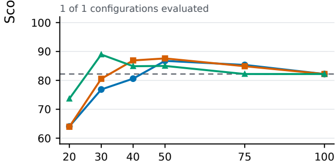
Multi-values NIAH
