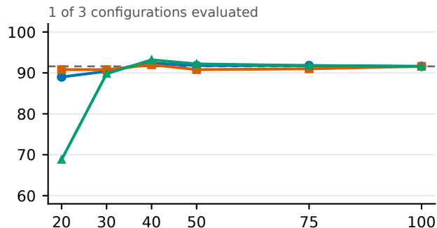
Multi-keys NIAH
