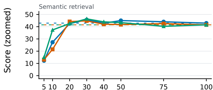
RepoQA (short)
