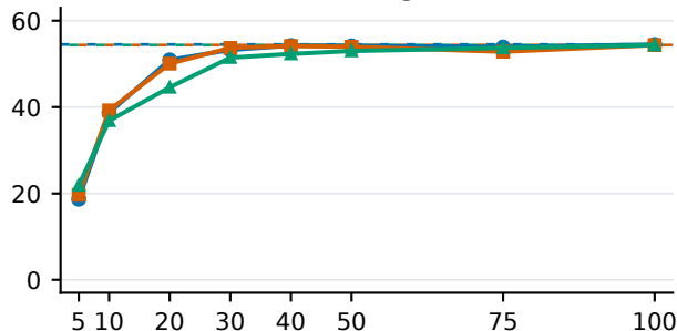
RULER: evaluated lengths
