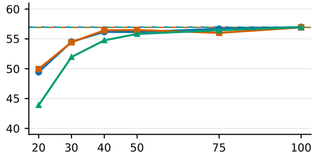
SCBench: all variants
