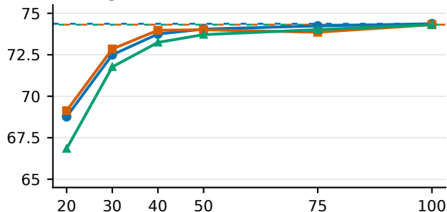
SCBench: all variants
