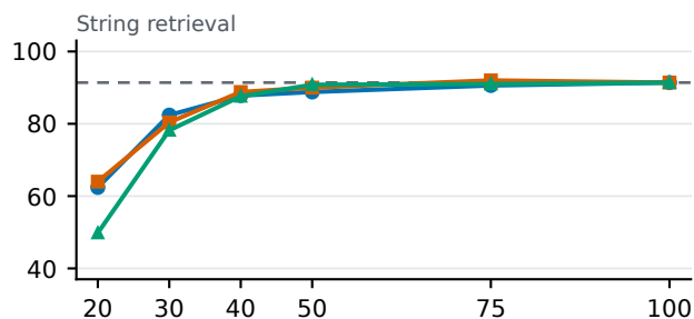
Summary + needles (base)
