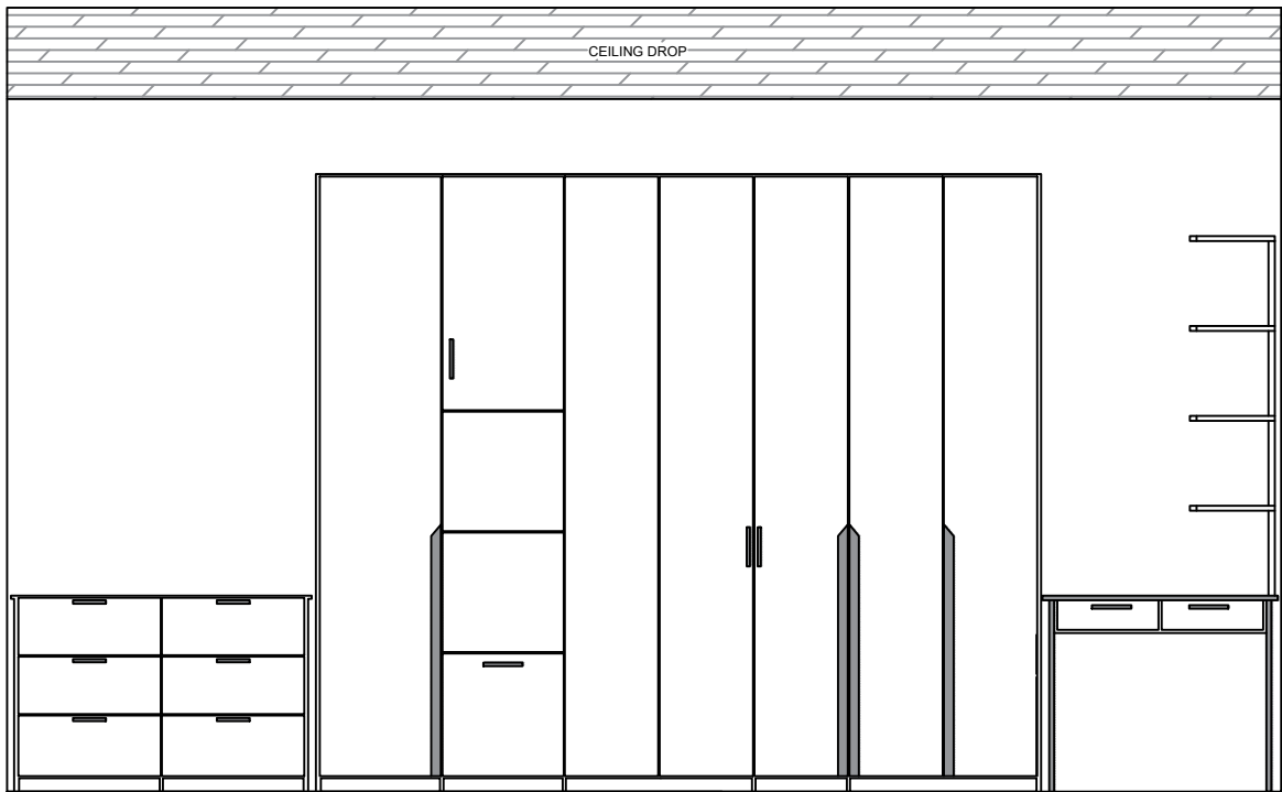
DRAWER, WARDROBE & STUDY TABLE DETAIL DRAWING
