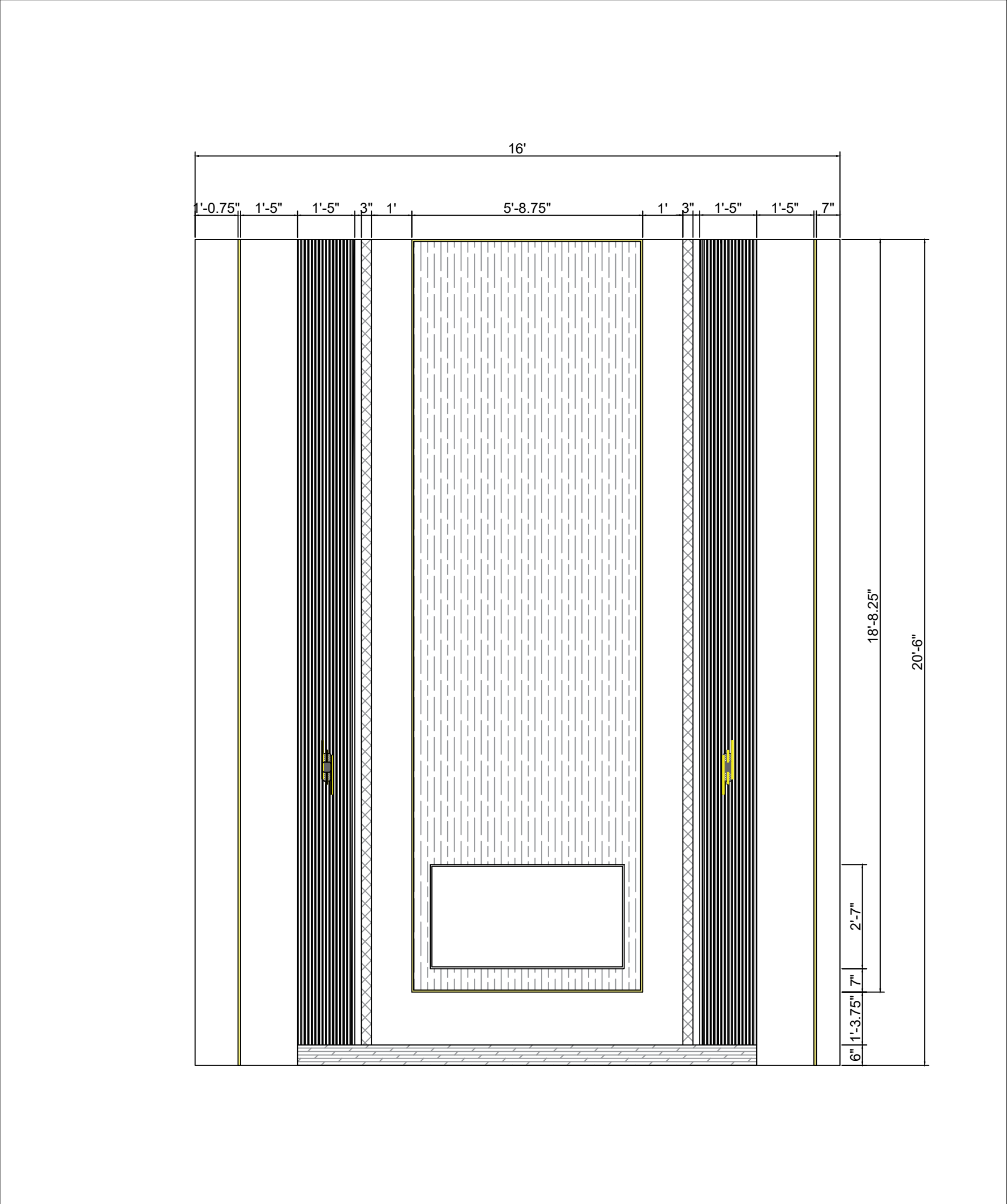
NORTH EAST WALL PENAL DETAIL DRAWING
