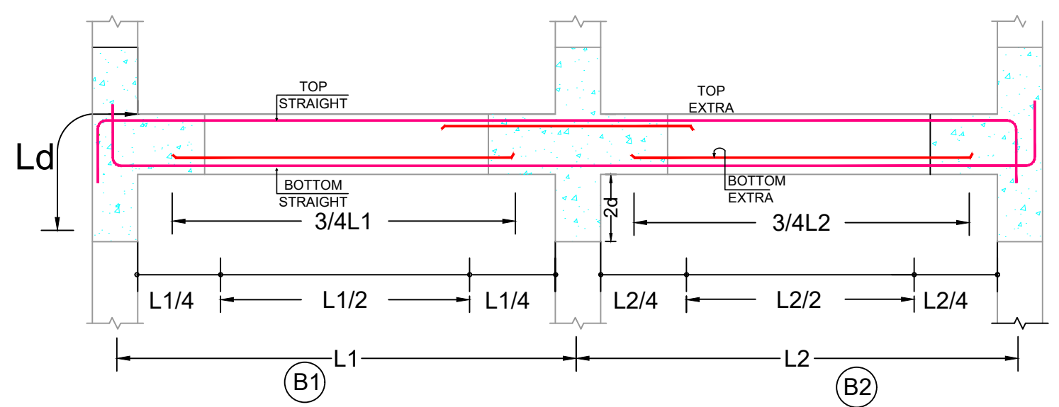
TYPICAL ARRANGEMENT OF BEAM REINFORCEMENT
