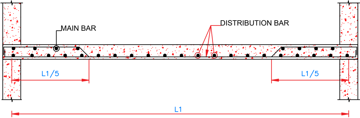
TYPICAL SECTION SHOWING SLAB REINFORCEMENT
