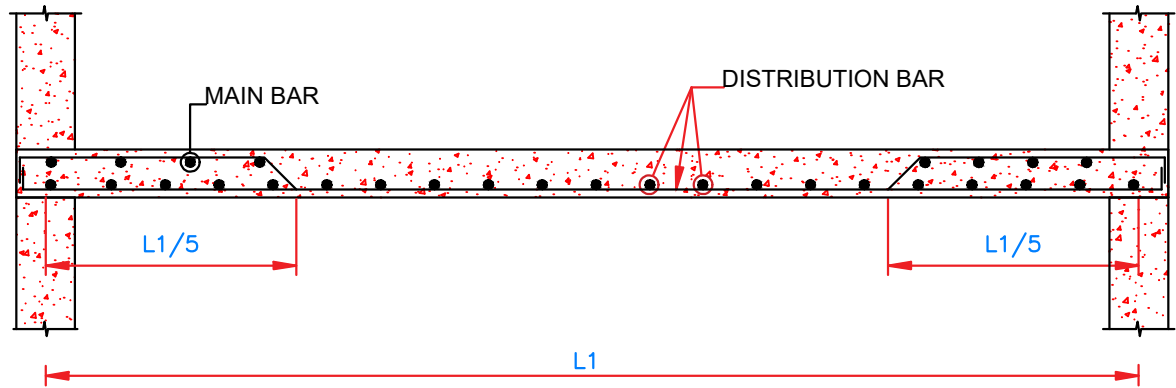
TYPICAL SECTION SHOWING SLAB REINFORCEMENT
