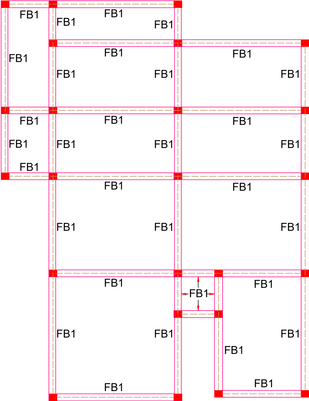
FLOOR BEAM LAYOUT
