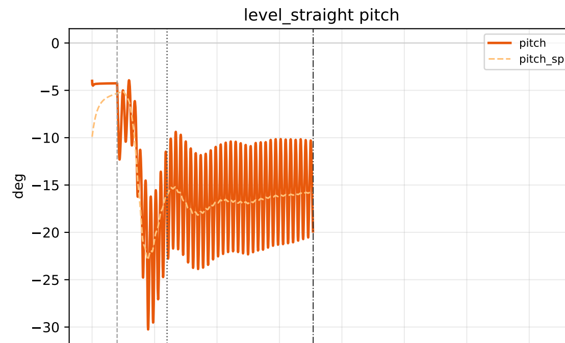
Canonical Attitude Curves: default COM=-0.10, tail=0.5/1.2
