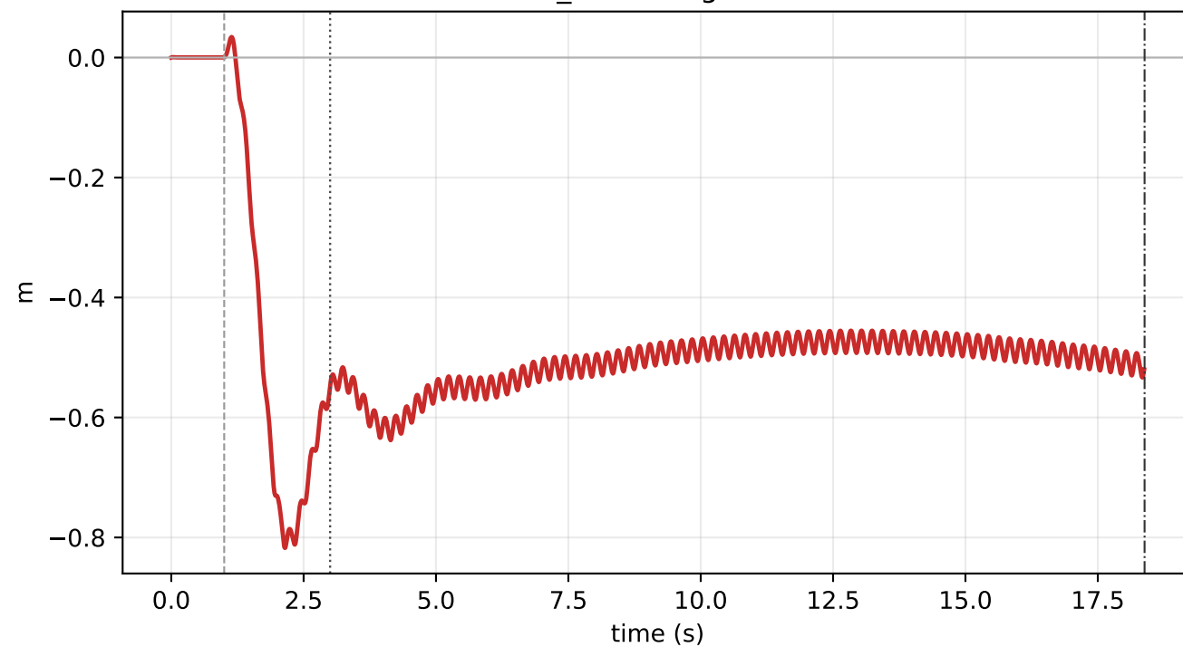
level_loiter height error
