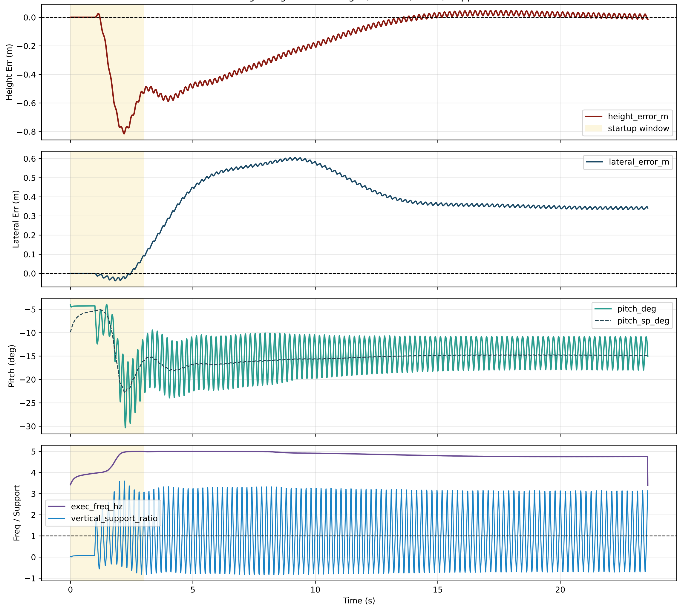
Long Straight 180m: Height / Lateral / Pitch / Support
