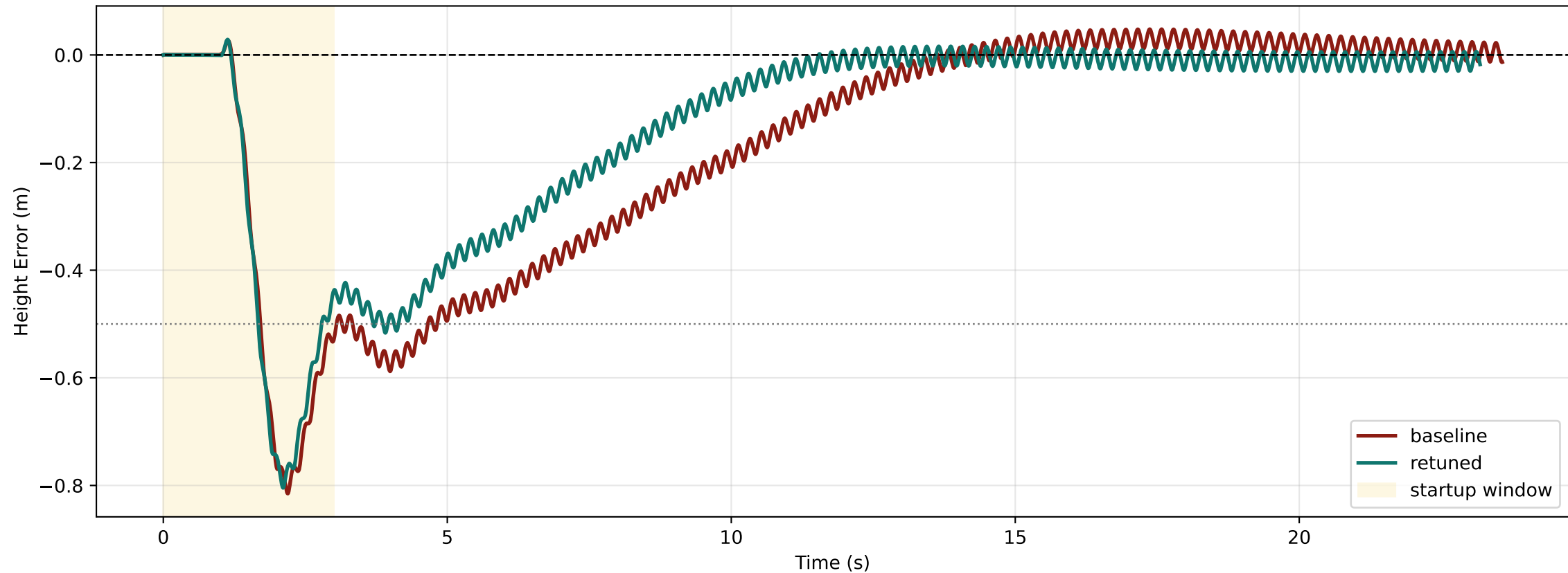
Long Straight 180m Height Error: Baseline vs Retuned Default
