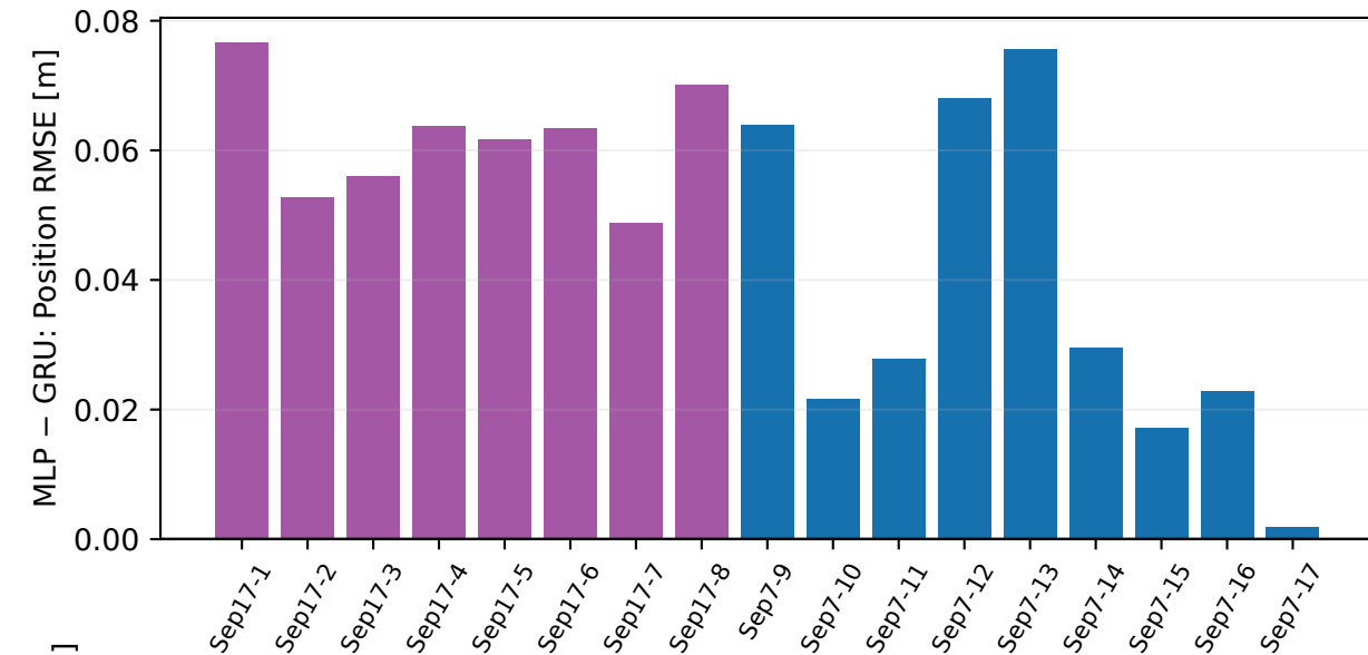
500 ms paired flights; each flight error averaged across 3 seeds Positive = GRU lower error; all 17 flights shown
