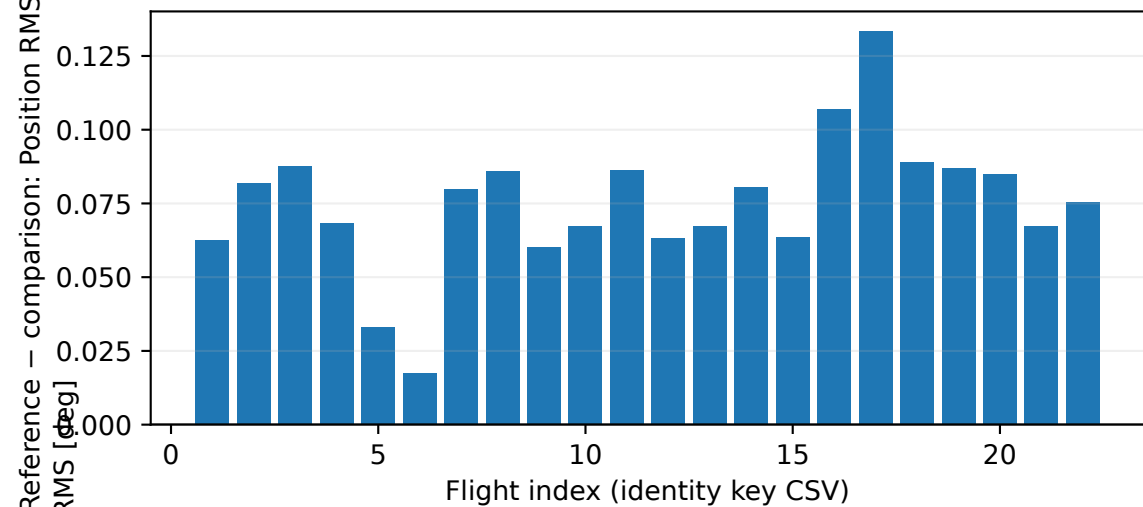
Sep19: GRU_vs_MLP, 500 ms; per-flight means across 3 seeds; positive favors comparison
