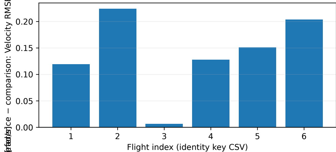
Sep8: GRU_vs_MLP, 500 ms; per-flight means across 3 seeds; positive favors comparison
