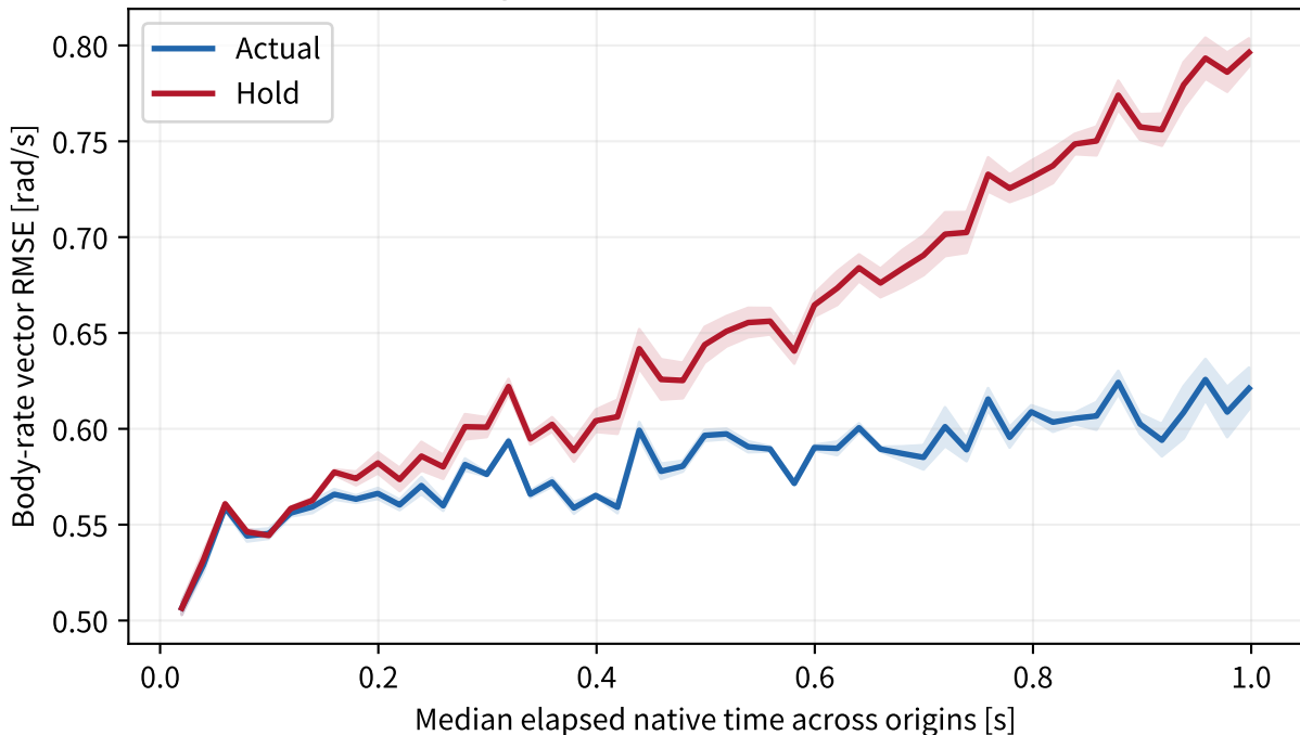
Equal-flight error; bands = \pm 1 seed SD (n=3)
