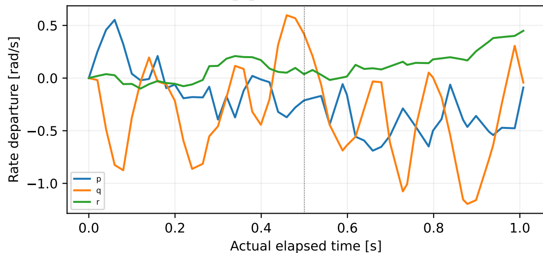
log_15_2026-9-15-18-23-44.ulg:0:165
