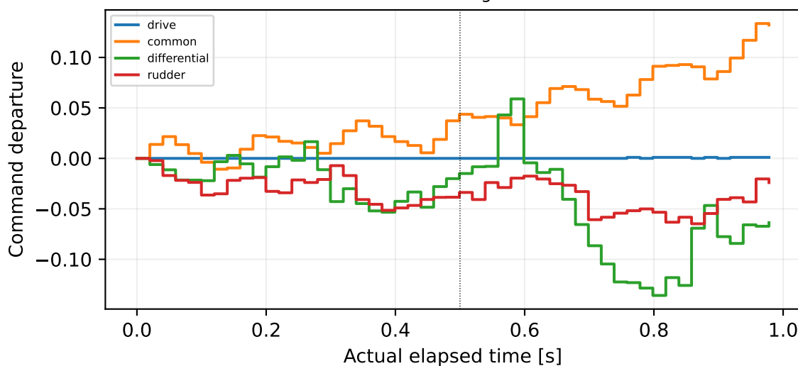
77: rudder sign=-1
