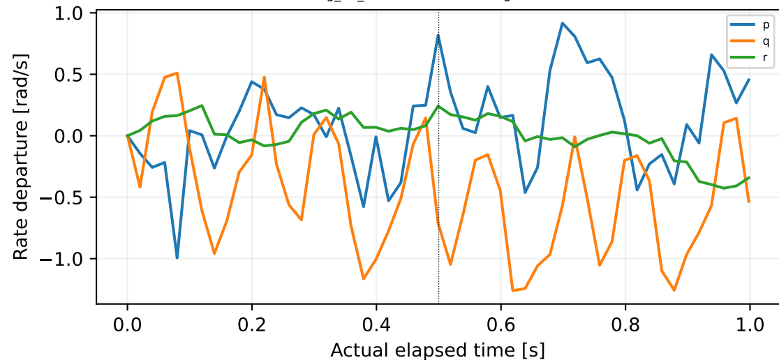
log_28_2026-9-6-07-01-38.ulg:8:115
