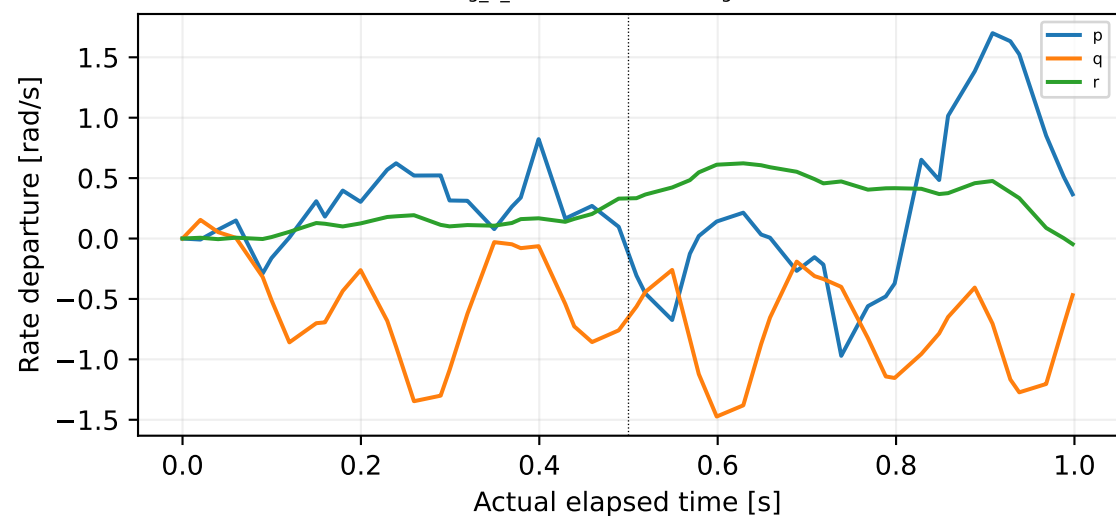
log_4_2026-9-16-18-20-50.ulg:0:135
