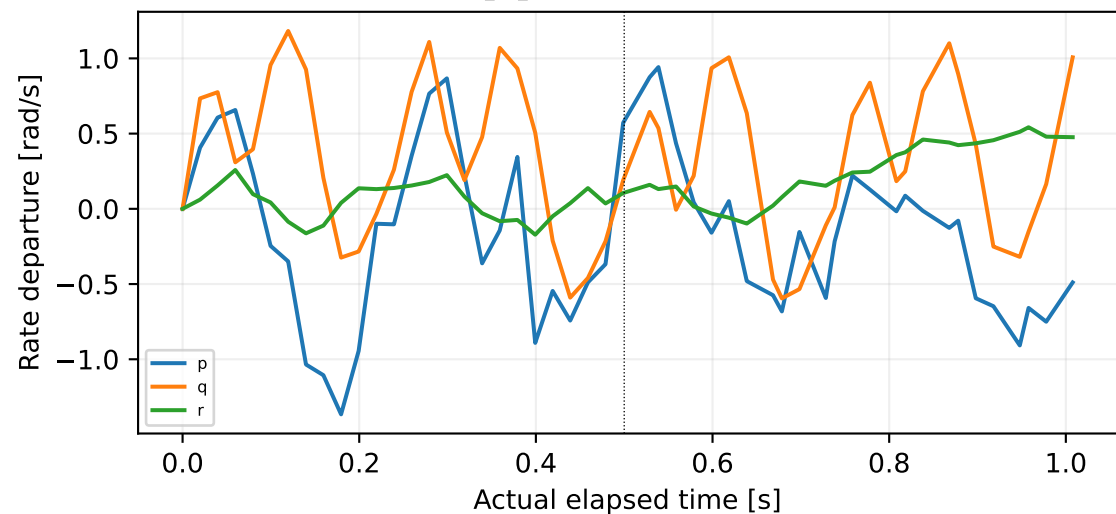
log_13_2026-9-11-18-28-08.ulg:2:375
