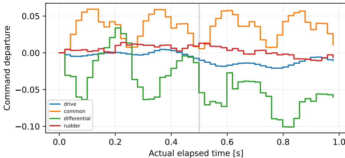
67: common sign=+1
