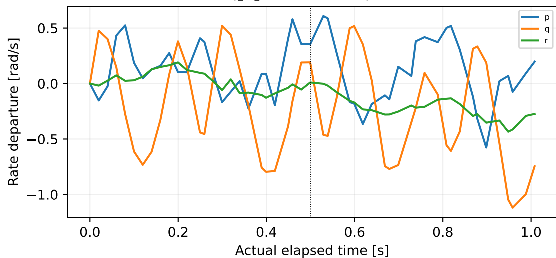
log_13_2026-9-15-18-10-58.ulg:2:405
