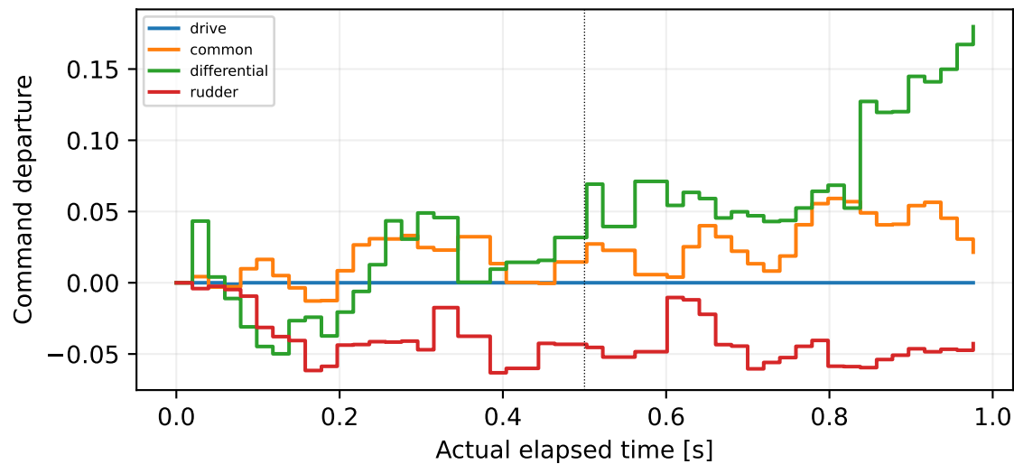
71: rudder sign=-1
