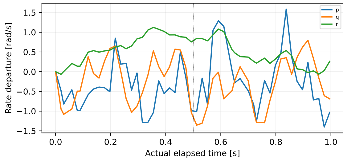
log_10_2026-9-12-06-13-40.ulg:1:215
