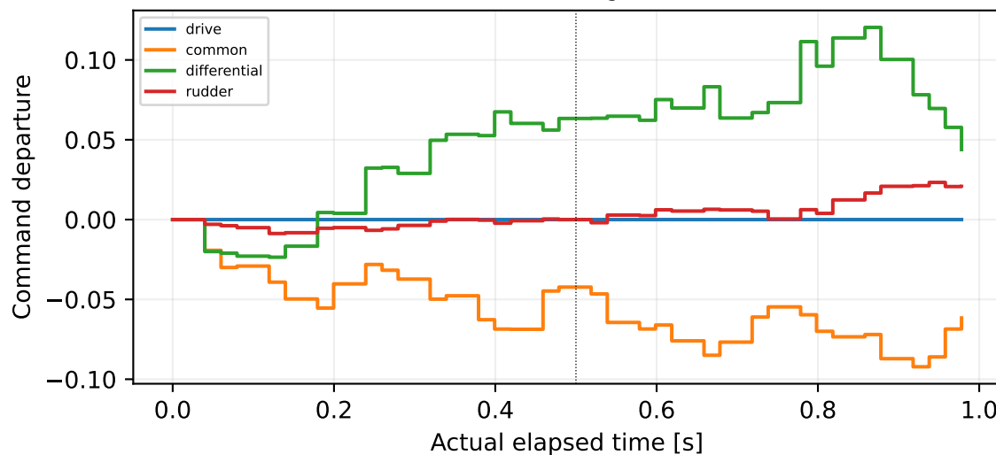
6: common sign=-1
