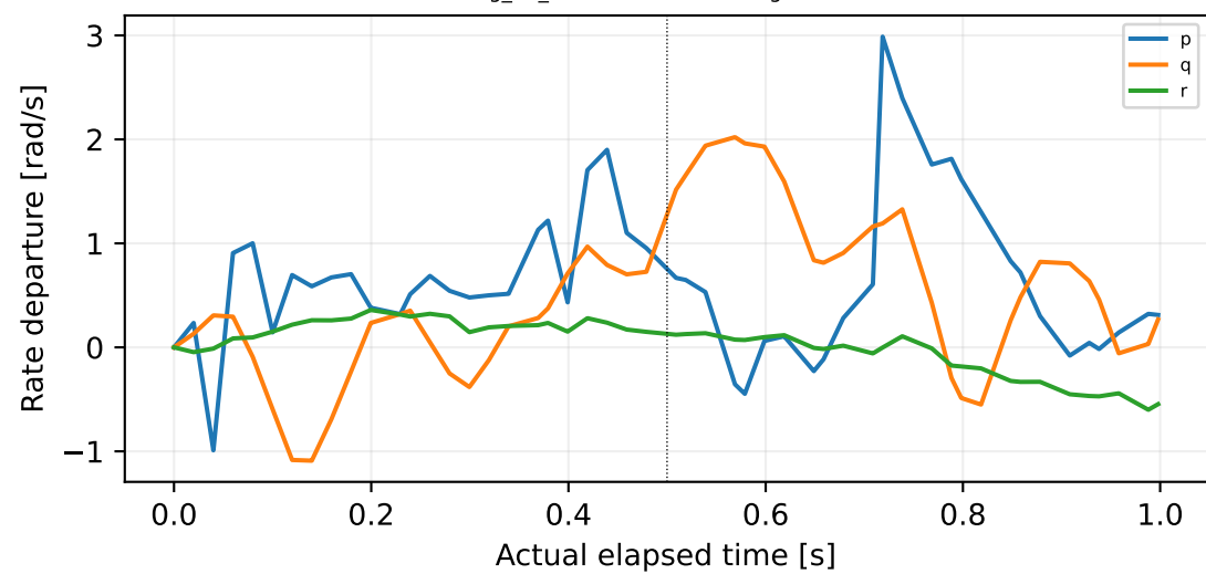
log_18_2026-9-6-18-46-20.ulg:0:845
