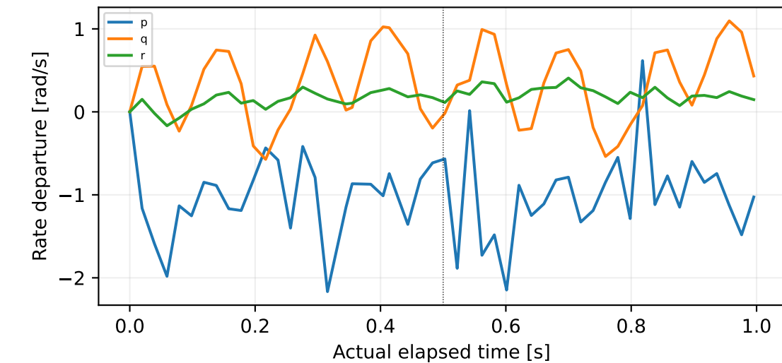
log_18_2026-9-6-18-46-20.ulg:6:1385
