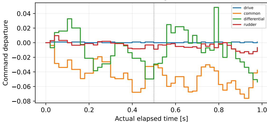
14: common sign=-1
