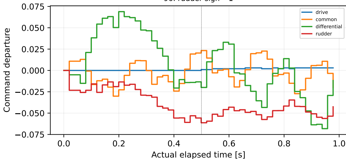
97: rudder sign=+1
