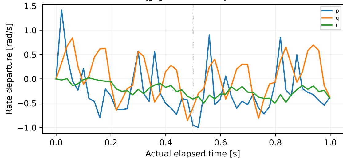
log_20_2026-9-6-18-58-10.ulg:0:1875
