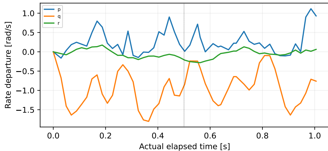
log_10_2026-9-12-06-13-40.ulg:0:315
