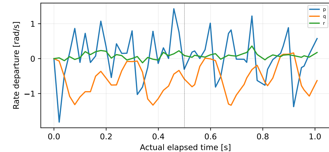
log_17_2026-9-6-18-34-06.ulg:2:1985
