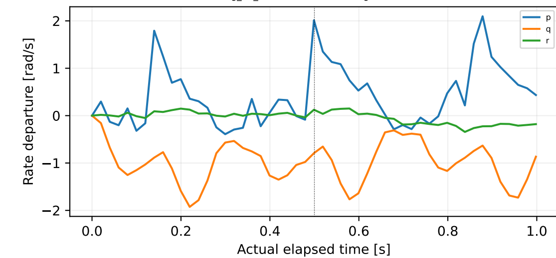
log_13_2026-9-14-18-28-32.ulg:3:185
