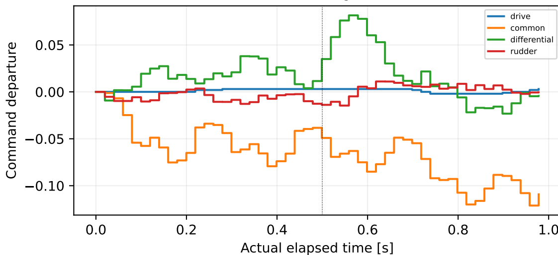
66: common sign=+1
