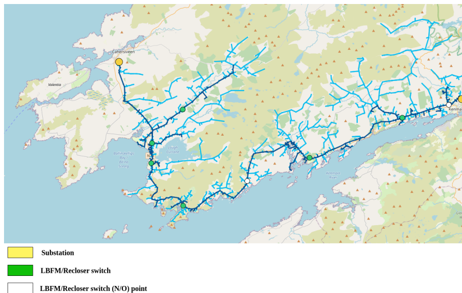
Figure 11: Kerry trial site circuitry and visualisation
