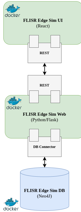
Figure 9: FLISR Edge simulation platform architecture
