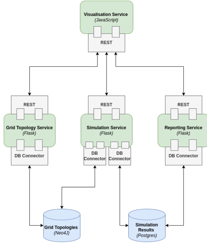
Figure 4: FLISR simulation platform architecture
