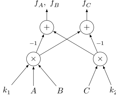
Figure 1: Expression graph of f_A = f_B = -k_1AB + k_2C and f_C = k_1AB - k_2C ; edge labels are coefficients.
