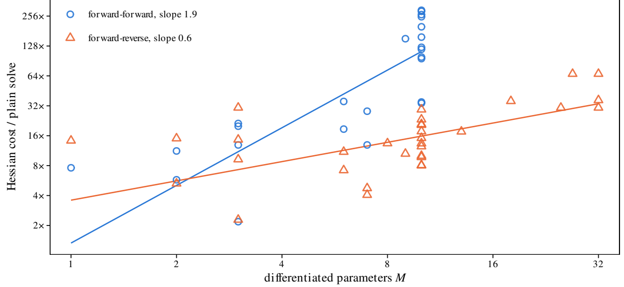
Figure 3: Cost of one Hessian of the summed outputs in units of the plain solve, one marker per problem and mode, geometric mean over the three tolerances. The lines are power laws fitted in log-log over M > 1 ; their exponents are given in the legend.
