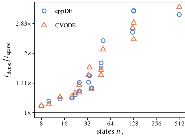
Figure 4: Gain of the sparse over the dense linear solver, one marker per model and backend, geometric mean over tolerances and modes.
