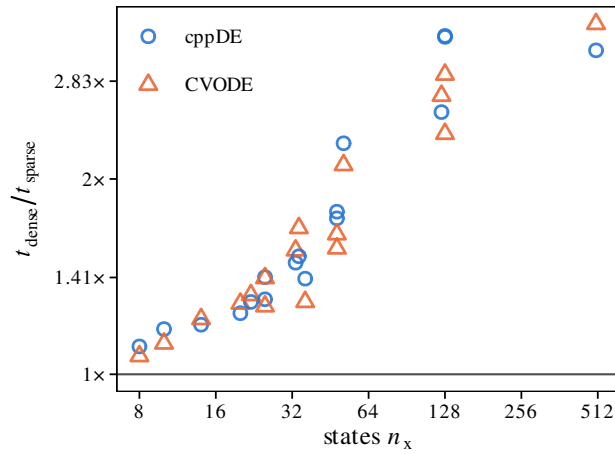
Figure 6: Gain of the sparse over the dense linear solver, one marker per model and backend.
