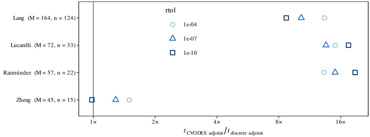
Figure 4: Time of one gradient by the CVODES adjoint over the time by the discrete adjoint, per model and tolerance; right of the line the discrete adjoint is faster.
