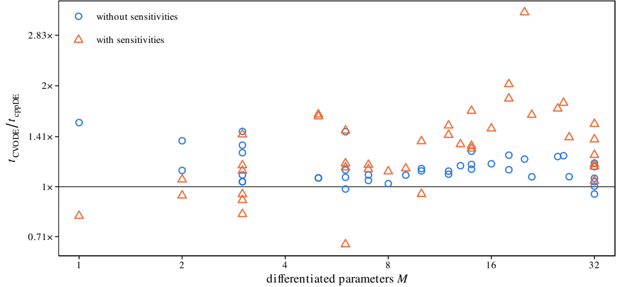
Figure 2: Head-to-head ratio of the two backends, one marker per problem and mode; above the line cppODE() is faster. The plain solve is placed at the M of its sensitivity counterpart.
