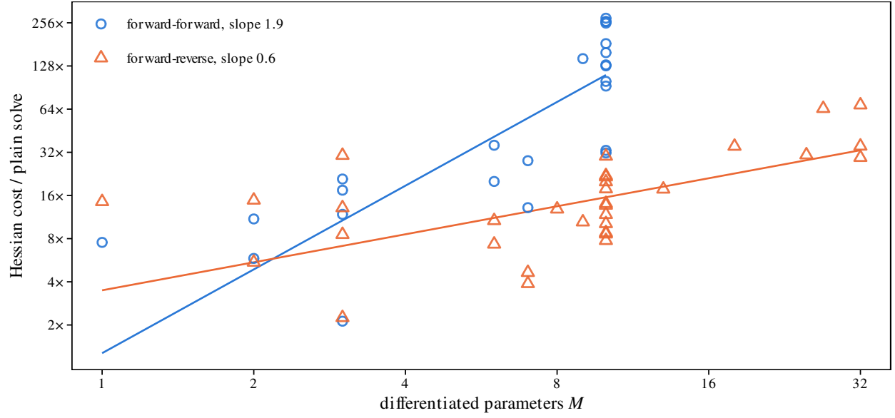
Figure 5: Cost of one Hessian of the summed outputs in units of the plain solve. The lines are power laws fitted in log-log over M > 1 .
