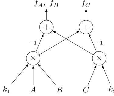
Figure 1: Expression graph of f_A = f_B = -k_1AB + k_2C and f_C = k_1AB - k_2C ; edge labels are coefficients.
