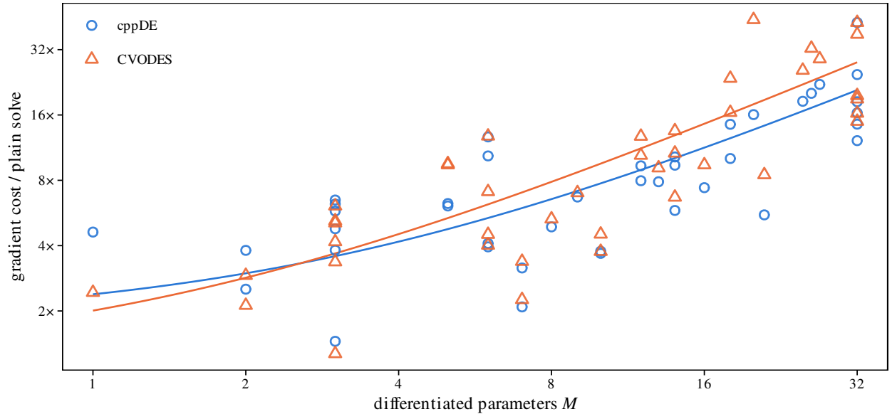
Figure 3: Cost of one gradient by forward sensitivities in units of the plain solve of the same problem and backend, with least-squares lines.
