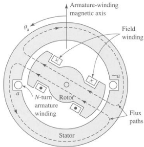
Figure 22: A simple diagram of a 2-pole salient generator.
