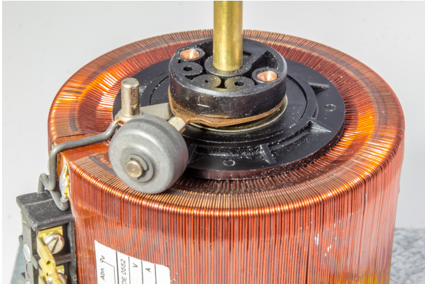
Figure 16: Variable autotransformer 0-220 V, 4 A, 880 VA.
