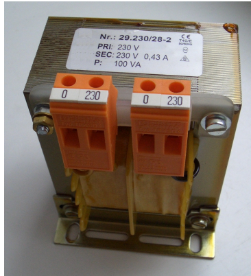
Figure 17: A 230 V isolation transformer.
