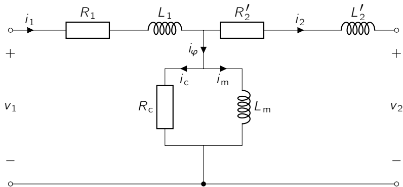
Figure 12: The equivalent circuit for a transformer.
