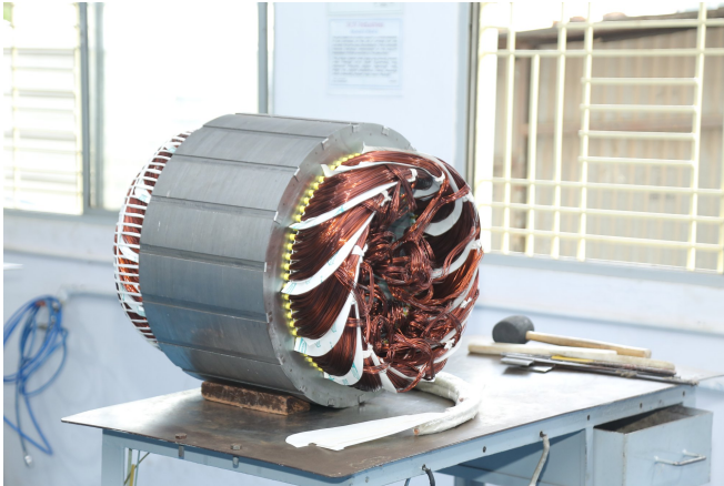
Figure 19: The armature of a AC is the stator as the stator has AC flowing during operation [19].
