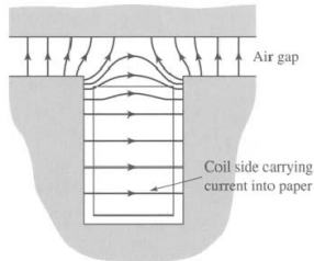
Figure 29: Flux created by a single coil side in a slot.
