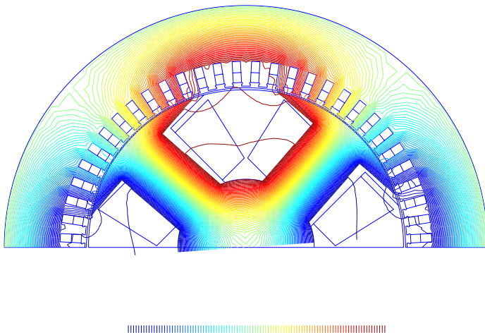
Figure 25: Finite-element solution for the flux distribution around a salient pole.
