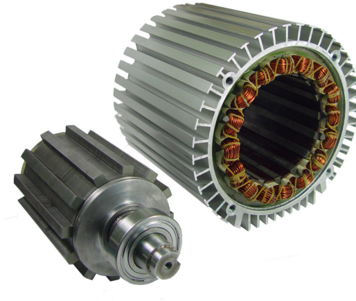
Figure 21: An example of a switched reluctance drive with its rotor (left) and stator (right).
