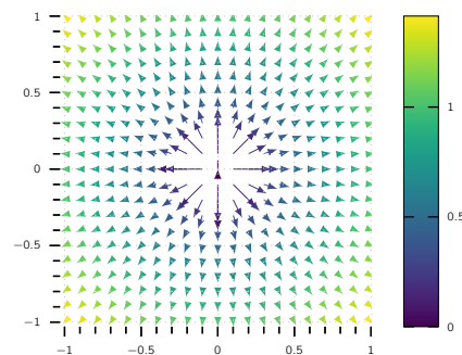
Figure 2.10 The vector plot of the "divergence problem".
