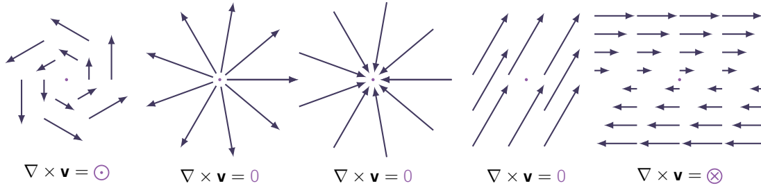
Figure 2.5 Different behaviours of the curl operation.
