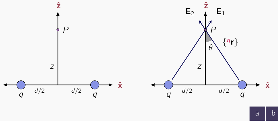
Figure 3.2: The diagram for the question “Electric Field at a Distance” (a) The geometrical description (b) Additional annotations added.
