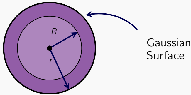
Figure 3.6: An imaginary Gaussian sphere.
