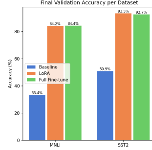
Figure 2: Bar chart summarizing our validation accuracy. We include the baseline (no fine-tuning) to show that without any fine tuning, the model is effectively guessing at random.
