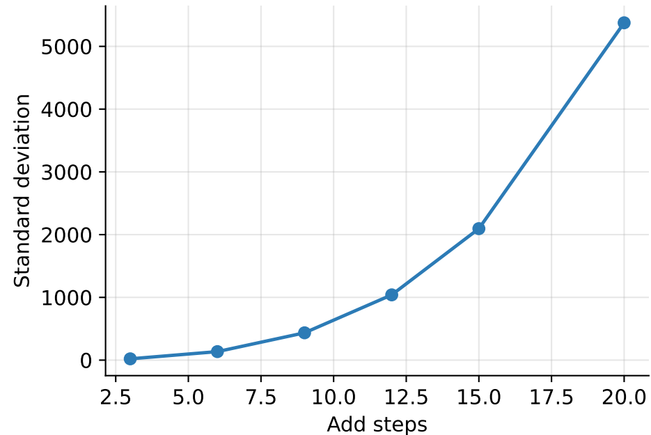
(a) Std vs program length
