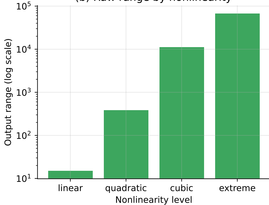
(b) Raw range by nonlinearity
