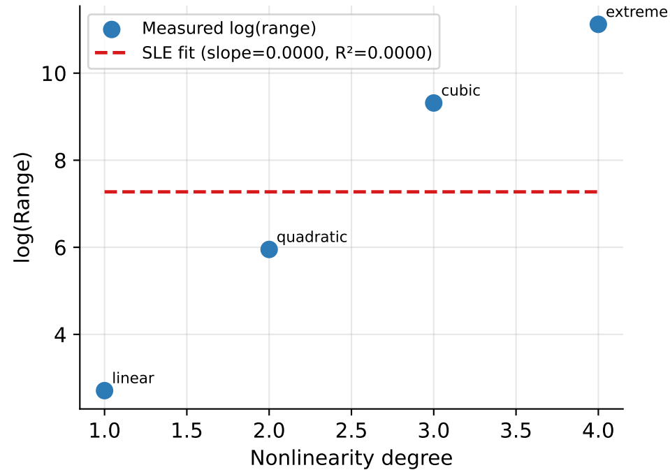
(a) SLE: log(range) vs nonlinearity degree
