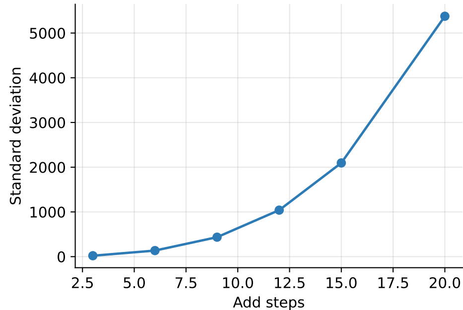
(a) Std vs program length
