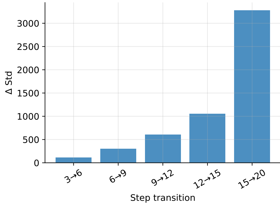
(b) Marginal \Delta std (non-decreasing = compounding)
