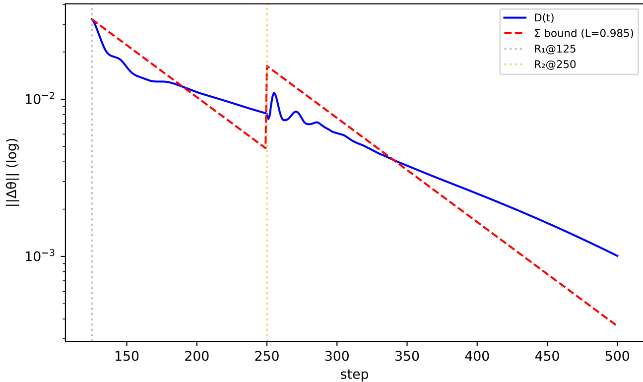
Plot 3: Compositional Bound [contractive]
