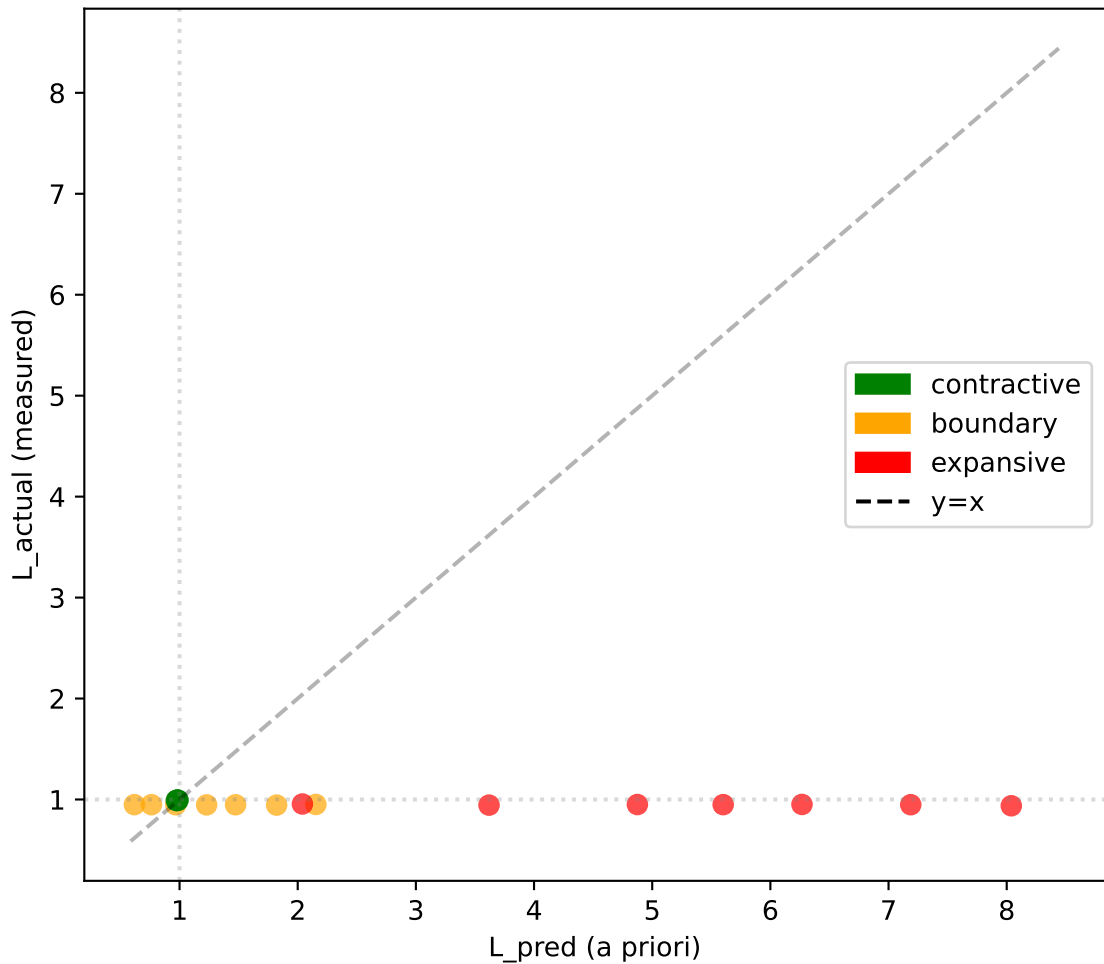
Plot 8: Prediction Accuracy
