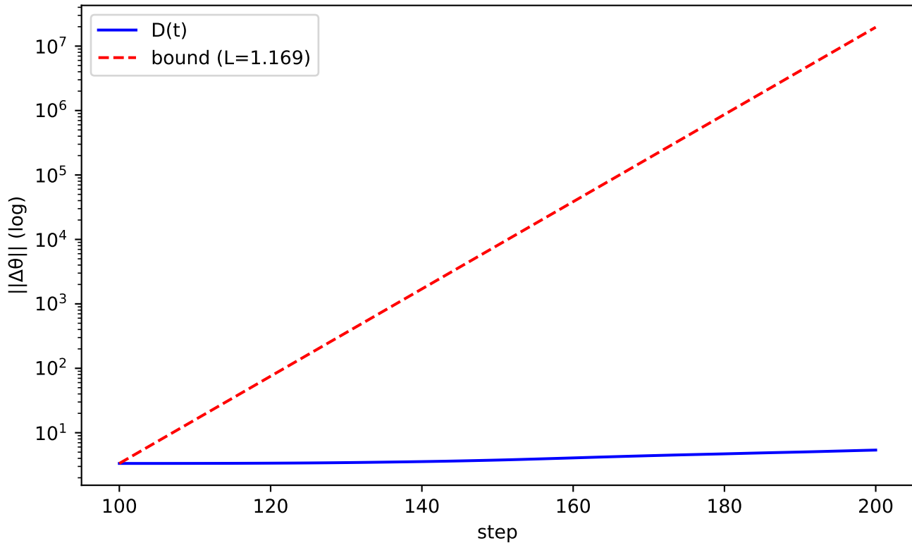
Plot 9: resnet18 (11181642 params) [expansive]
