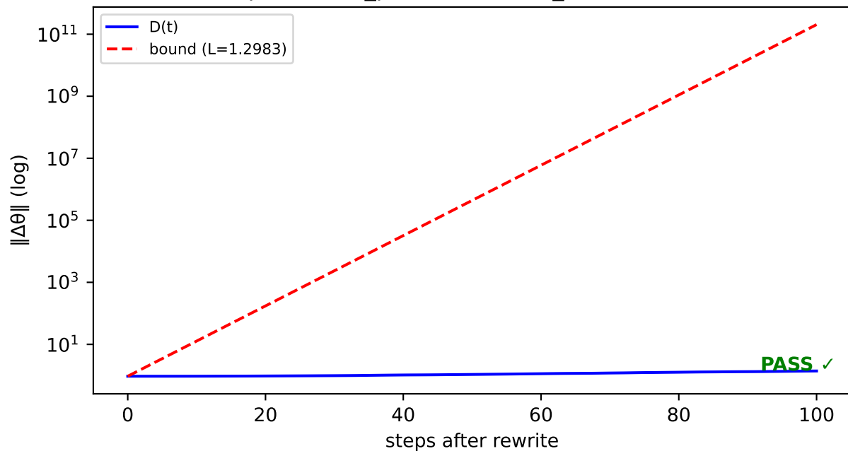
Plot 9C: GPT-mini (881,792 params) [expansive] L_pred=1.2983, L_actual=1.0039
