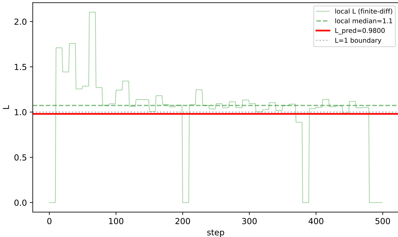
Plot 4: Local vs A Priori Lipschitz
