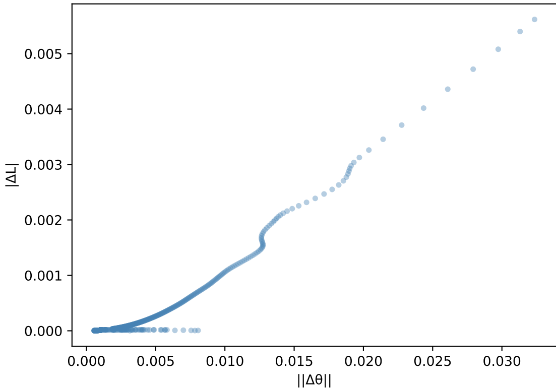
Plot 6: Loss Gap vs \theta -Divergence ( \rho=0.936 )
